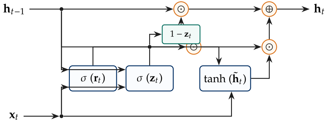
Figure 4.3: The Gated Recurrent Unit (GRU) cell architecture. Reset gate \mathbf{r}_t dynamically filters previous hidden state \mathbf{h}_{t-1} before constructing candidate state \tilde{\mathbf{h}}_t . Update gate \mathbf{z}_t controls the convex interpolation (1 - \mathbf{z}_t) \odot \mathbf{h}_{t-1} + \mathbf{z}_t \odot \tilde{\mathbf{h}}_t , unifying long- and short-term memory into a single state vector \mathbf{h}_t .
