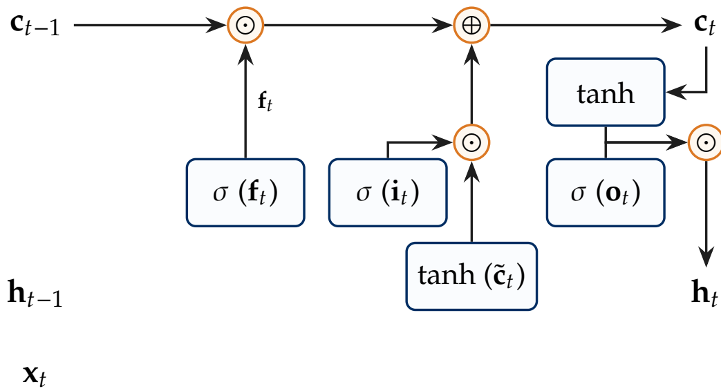
Figure 4.2: The LSTM memory cell architecture. The top horizontal path forms the uninterrupted additive cell state highway \mathbf{c}_t (the Constant Error Carousel). Forget gate f_t , input gate i_t , and output gate o_t modulate information flow using multiplicative valves.
