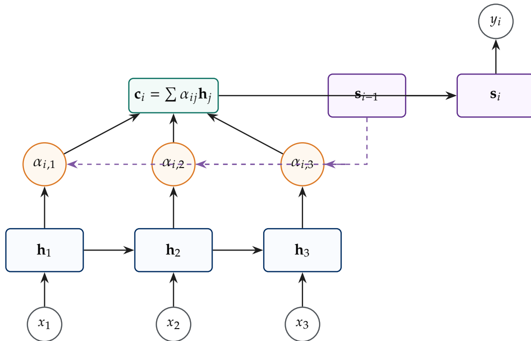
Figure 4.5: The Bahdanau Additive Attention mechanism. At decoder step i , previous decoder state \mathbf{s}_{i-1} is compared against all encoder annotations \mathbf{h}_j via Equation (4.27), producing attention distribution \alpha_{ij} . The weighted sum synthesizes dynamic context vector \mathbf{c}_i \in \mathbb{R}^{2d_h} , directly feeding relevant source features into decoder state \mathbf{s}_i .
