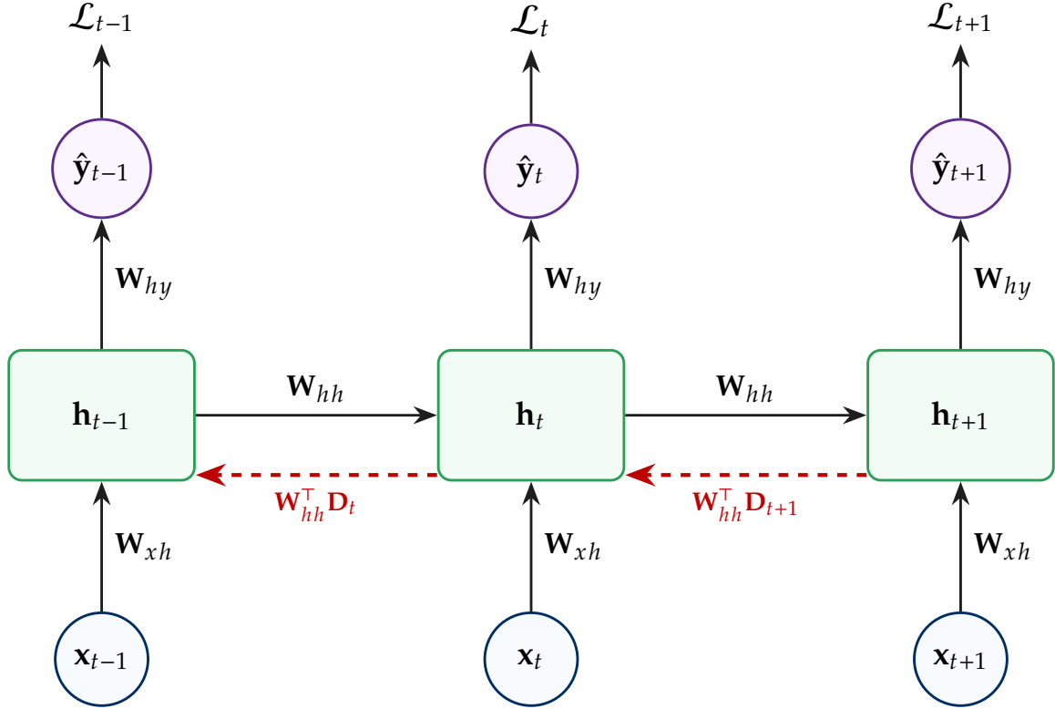
Figure 4.1: Unrolling an RNN cell across time steps t - 1, t, t + 1 . Solid black arrows show the forward propagation of inputs \mathbf{x}_t and recurrent states \mathbf{h}_t . Dashed red arrows trace Backpropagation Through Time (BPTT), where gradients accumulate across time via repeated multiplications by the Jacobian \mathbf{W}_{hh}^\top \mathbf{D}_t .
