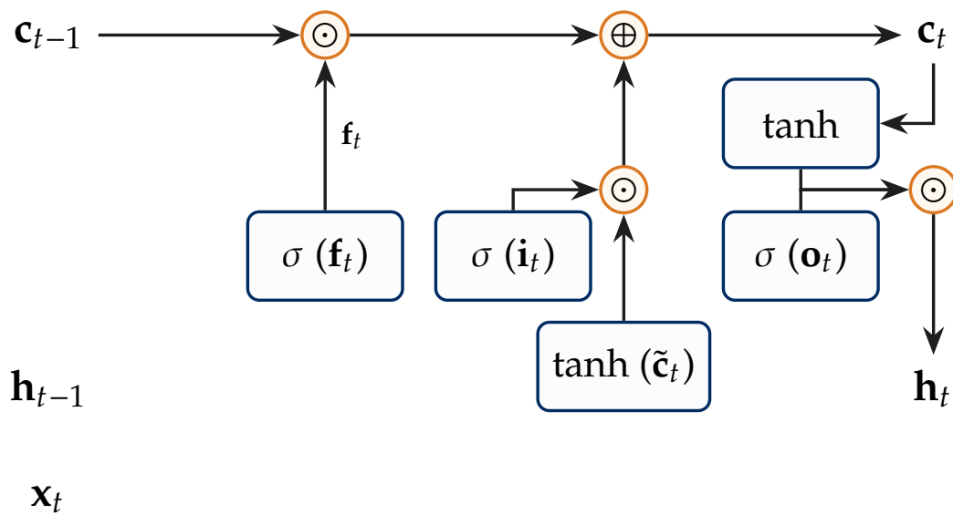
Figure 3.2: The LSTM memory cell architecture. The top horizontal path forms the uninterrupted additive cell state highway \mathbf{c}_t (the Constant Error Carousel). Forget gate \mathbf{f}_t , input gate \mathbf{i}_t , and output gate \mathbf{o}_t modulate information flow using multiplicative valves.
