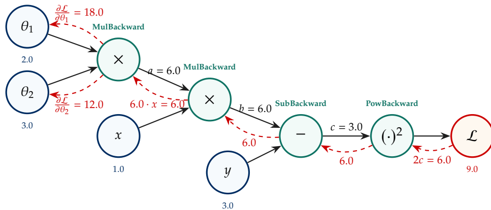
Figure 1.4: Vector rendering of the computational graph for Exercise 3 (reproducing the notebook’s computational_graph.png and backpropagation.png ). Black solid paths trace forward evaluation; red dashed arrows trace reverse-mode adjoint gradient propagation via the chain rule.
