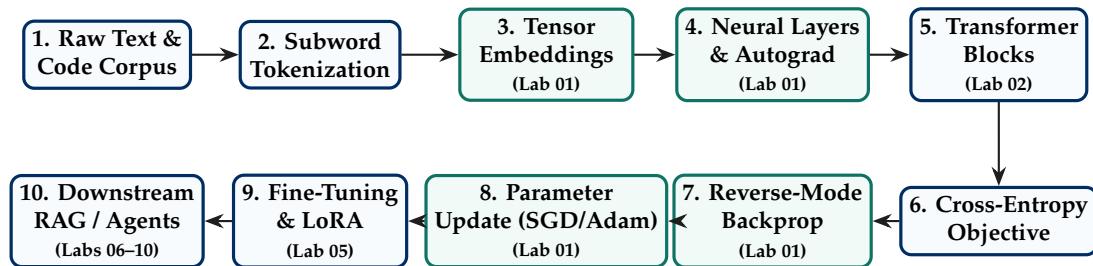
Figure 1.1: The end-to-end lifecycle of Large Language Models. Laboratory 01 establishes the atomic computational substrate: multidimensional tensors (Step 3), modular neural layers and forward graphs (Step 4), reverse-mode autograd (Step 7), and iterative optimization loops (Step 8).
