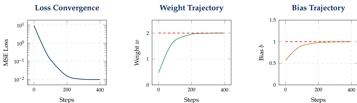
Figure 1.2: Visualizing optimization dynamics across 50 epochs (Cell 25). The mean squared error decays logarithmically towards the irreducible noise floor ( \sigma^2 = 0.01 ), while weight w asymptotically reaches 2.0 and bias b reaches 1.0.
