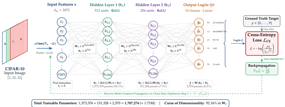
Figure 1.3: Architectural topology of the SimpleNN Multi-Layer Perceptron (MLP) for CIFAR-10 classification (Section 1.6.1). An input color image [3 \times 32 \times 32] is flattened into feature vector x \in \mathbb{R}^{3072} , sequentially propagated through two hidden fully-connected layers with non-linear ReLU activations (512 and 256 units), and projected into 10 unnormalized class logits \hat{y} \in \mathbb{R}^{10} . Training is supervised by Cross-Entropy Loss with gradients propagated in reverse mode.
