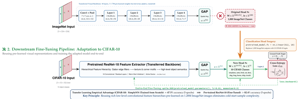
Figure 1.4: Architectural topology of transfer learning and fine-tuning with ResNet-18 on CIFAR-10 (Section 1.7.2). (Top) The source ResNet-18 model pre-trained on ImageNet-1K (1.28M images, 1,000 categories) features 18 residual convolutional layers and an original 1,000-class classification head. (Middle) Classification head surgery replaces pretrained_model.fc with a new linear projection W \in \mathbb{R}^{10 \times 512} , b \in \mathbb{R}^{10} . (Bottom) End-to-end downstream fine-tuning on CIFAR-10 ( [3 \times 32 \times 32] ), propagating gradients through both the new head and the pre-trained feature extractor, boosting classification accuracy from 47.5% (MLP from scratch) to > 82.4\% in just 5 epochs.
