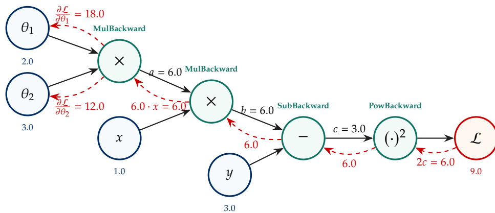
Figure 1.5: Vector rendering of the computational graph for Exercise 3 (reproducing the notebook’s computational_graph.png and backpropagation.png ). Black solid paths trace forward evaluation; red dashed arrows trace reverse-mode adjoint gradient propagation via the chain rule.
