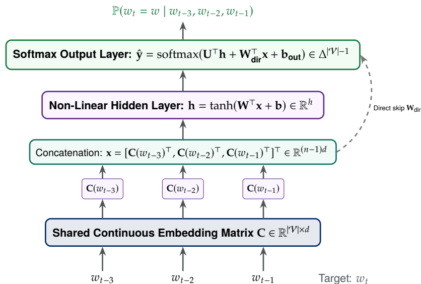
Figure 1.6: Yoshua Bengio's Neural Probabilistic Language Model (NPLM, 2003). Discrete context words are mapped into continuous dense feature vectors via shared matrix \mathbf{C} \in \mathbb{R}^{|\mathcal{V}| \times d} , concatenated, and processed through a non-linear hidden layer to predict next-token probabilities via softmax.
