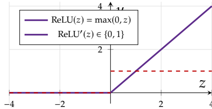
(c) Rectified Linear Unit (ReLU)
