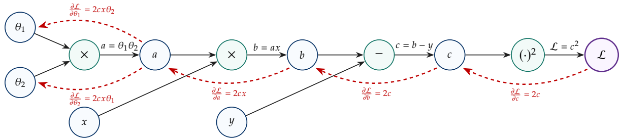
Figure 2.9: Directed Acyclic Computational Graph (DAG) for model \hat{y} = \theta_1 \theta_2 x with quadratic loss \mathcal{L} = (\theta_1 \theta_2 x - y)^2 (reproduced from Slide 24). Solid black arrows trace forward execution; dashed red arrows trace reverse-mode adjoint backpropagation via the chain rule [21].
