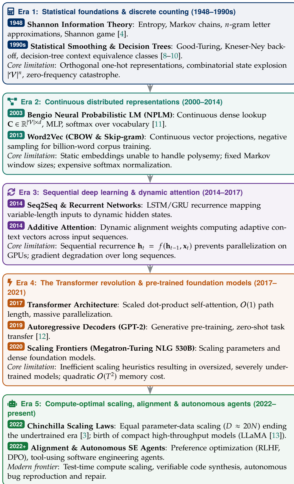
Figure 1.3: Chronological timeline of language model evolution from 1948 to the present.
