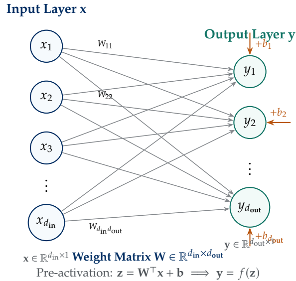
Figure 2.4: Architecture of a fully connected dense layer mapping an input vector \mathbf{x} \in \mathbb{R}^{d_{\text{in}}} to output \mathbf{y} \in \mathbb{R}^{d_{\text{out}}} . Each directed edge carries an individual scalar weight W_{ij} , and each output neuron incorporates an additive bias b_j .
