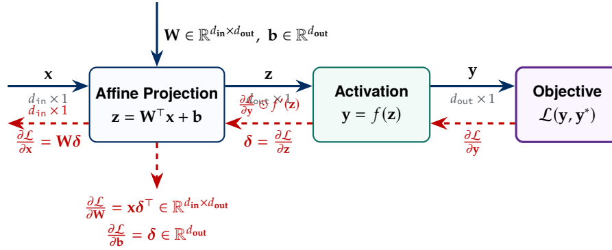
Figure 2.10: Vectorized matrix adjoint backpropagation across a fully connected dense layer. Solid navy arrows trace forward execution mapping input \mathbf{x} \in \mathbb{R}^{d_{\text{in}}} to output \mathbf{y} \in \mathbb{R}^{d_{\text{out}}} ; dashed red arrows trace reverse-mode adjoint error propagation ( \boldsymbol{\delta} \in \mathbb{R}^{d_{\text{out}}} ), yielding parameter updates \frac{\partial \mathcal{L}}{\partial \mathbf{W}} = \mathbf{x} \boldsymbol{\delta}^\top , \frac{\partial \mathcal{L}}{\partial \mathbf{b}} = \boldsymbol{\delta} , and upstream gradient \frac{\partial \mathcal{L}}{\partial \mathbf{x}} = \mathbf{W} \boldsymbol{\delta} .
