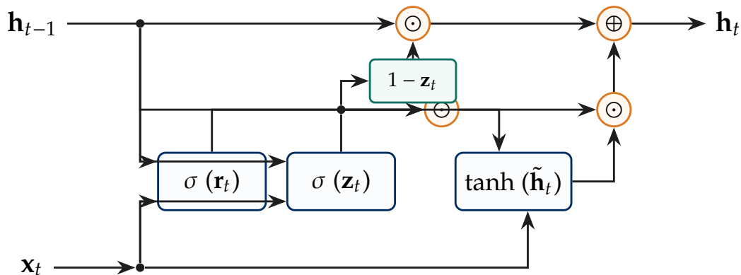
Figure 3.3: The Gated Recurrent Unit (GRU) cell architecture. Reset gate \mathbf{r}_t dynamically filters previous hidden state \mathbf{h}_{t-1} before constructing candidate state \tilde{\mathbf{h}}_t . Update gate \mathbf{z}_t controls the convex interpolation (1 - \mathbf{z}_t) \odot \mathbf{h}_{t-1} + \mathbf{z}_t \odot \tilde{\mathbf{h}}_t , unifying long- and short-term memory into a single state vector \mathbf{h}_t .
