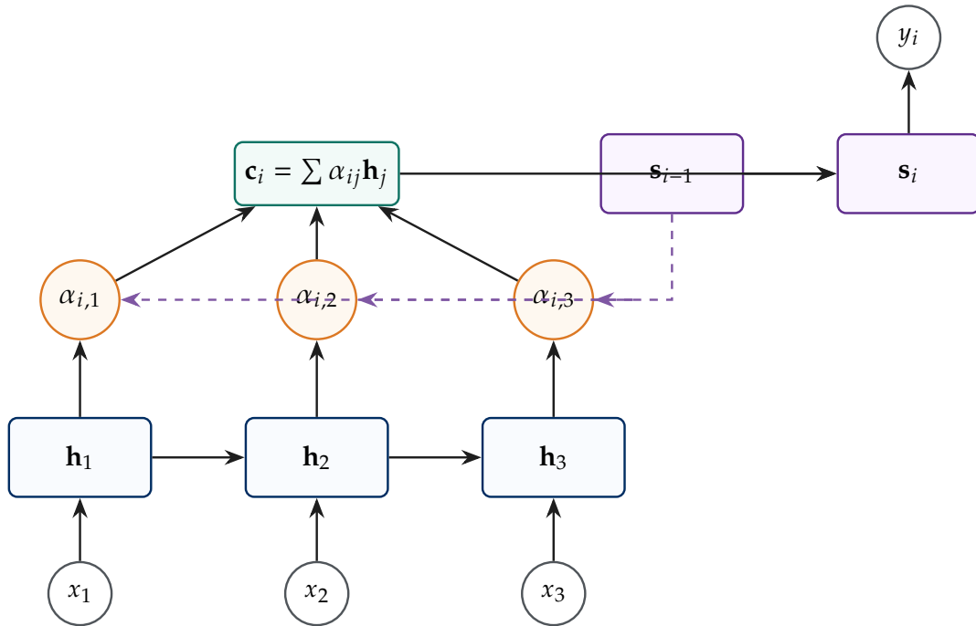
Figure 3.5: The Bahdanau Additive Attention mechanism. At decoder step i , previous decoder state \mathbf{s}_{i-1} is compared against all encoder annotations \mathbf{h}_j via Equation (3.27), producing attention distribution \alpha_{ij} . The weighted sum synthesizes dynamic context vector \mathbf{c}_i \in \mathbb{R}^{2d_h} , directly feeding relevant source features into decoder state \mathbf{s}_i .
