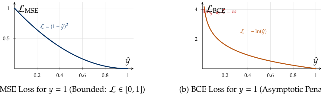
Figure 2.8: Comparison of loss function behaviors for target y = 1 . While MSE is bounded quadratically at 1.0, BCE imposes an asymptotic infinite penalty ( \mathcal{L} \rightarrow \infty ) as predicted probability \hat{y} \rightarrow 0 , providing steep, non-vanishing corrective gradients.
