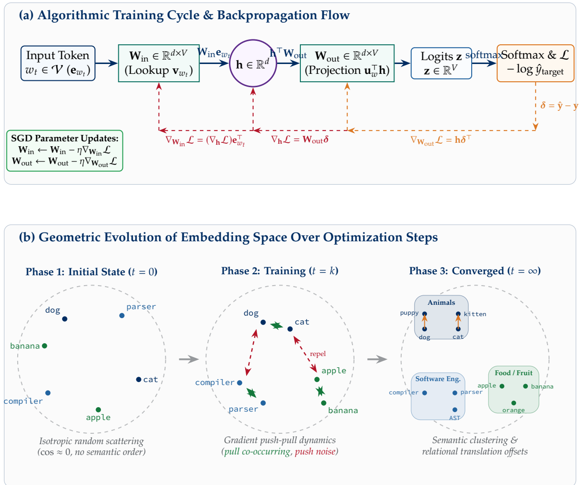
Figure 4.2: The embedding training loop and semantic space evolution. (a) Computational dataflow of the forward prediction pass and backward adjoint parameter updates. (b) Three-phase geometric evolution of embedding space from isotropic random scattering to clustered semantic topology with parallel relational offsets.
