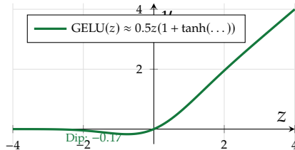
(e) Gaussian Error Linear Unit (GELU)
