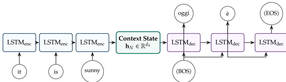
Figure 3.4: The Sequence-to-Sequence (Seq2Seq) Encoder-Decoder architecture. The Encoder LSTM compresses the variable-length source sentence into a single context state \mathbf{h}_N . The Decoder LSTM is initialized with \mathbf{h}_N and autoregressively emits target tokens from \langle \text{BOS} \rangle until emitting \langle \text{EOS} \rangle .
