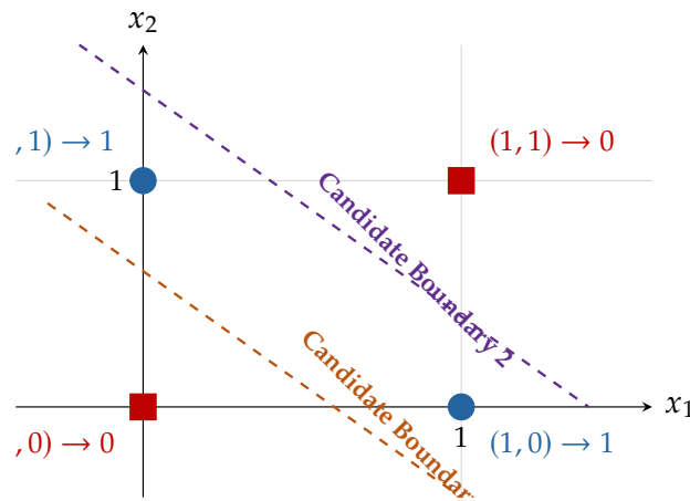
Figure 2.3: The XOR linear inseparability barrier (Minsky & Papert 1969). Class 1 points (0, 1) and (1, 0) (blue circles) cannot be separated from Class 0 points (0, 0) and (1, 1) (red squares) by any single linear hyperplane w_1x_1 + w_2x_2 + w_0 = 0 . Any single line either isolates (0, 0) or (1, 1), but cannot simultaneously group both off-diagonal points.
