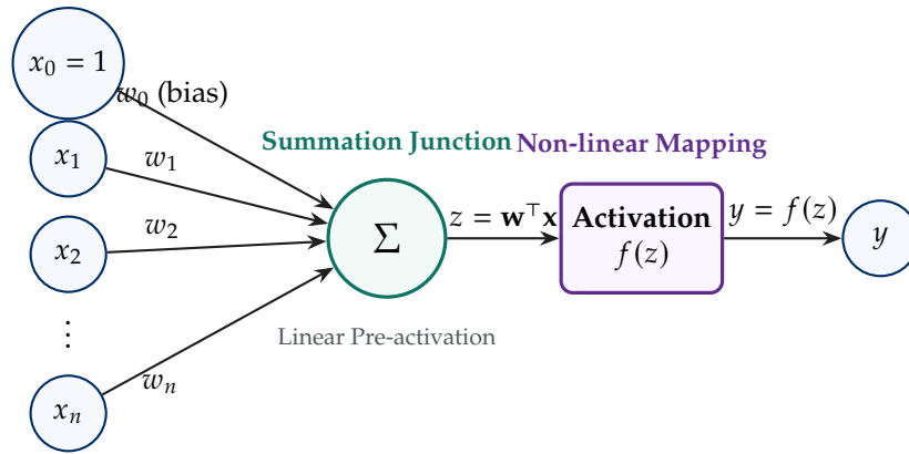
Figure 2.1: Architectural schematic of the artificial perceptron. Inputs x_i are modulated by synaptic weights w_i , accumulated with bias w_0 at the summation junction \Sigma to yield pre-activation z = \mathbf{w}^T \mathbf{x} , and mapped through activation function f(z) to produce scalar output y .
