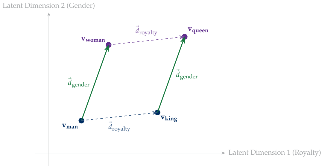
Figure 4.5: Geometric parallelogram in continuous embedding space demonstrating relational vector translations: \mathbf{v}_{\text{King}} - \mathbf{v}_{\text{Man}} \approx \mathbf{v}_{\text{Queen}} - \mathbf{v}_{\text{Woman}} . The directional displacement \vec{d}_{\text{gender}} isolates the feminine gender transformation, while \vec{d}_{\text{royalty}} isolates the monarchical status offset.
