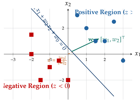
Figure 2.2: Geometric representation of the perceptron decision boundary in \mathbb{R}^2 . The line w_1x_1 + w_2x_2 + w_0 = 0 partitions feature space into positive ( \mathcal{H}^+ ) and negative ( \mathcal{H}^- ) half-spaces. The weight vector \mathbf{w} defines the normal vector to the separating hyperplane, and the scalar bias w_0 determines its distance from the origin.
