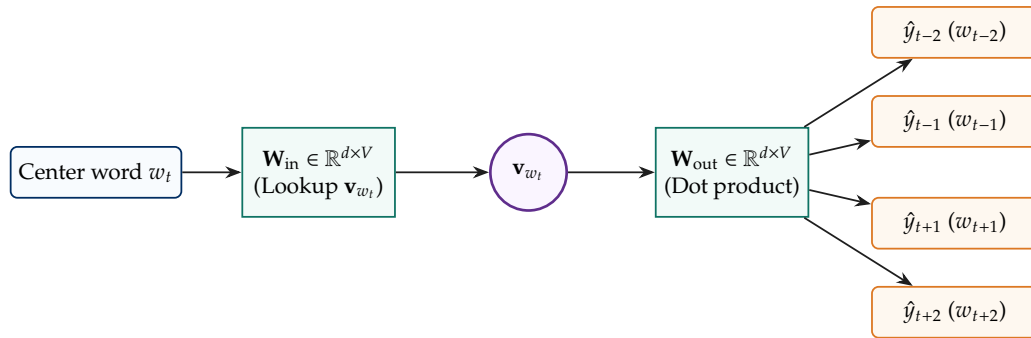
Figure 4.4: Continuous Skip-Gram architecture. A single center target word w_t is projected via \mathbf{W}_{\text{in}} \in \mathbb{R}^{d \times V} into vector \mathbf{v}_{w_t} \in \mathbb{R}^d , which predicts the probability distribution of context words across window radius c through output matrix \mathbf{W}_{\text{out}} .
