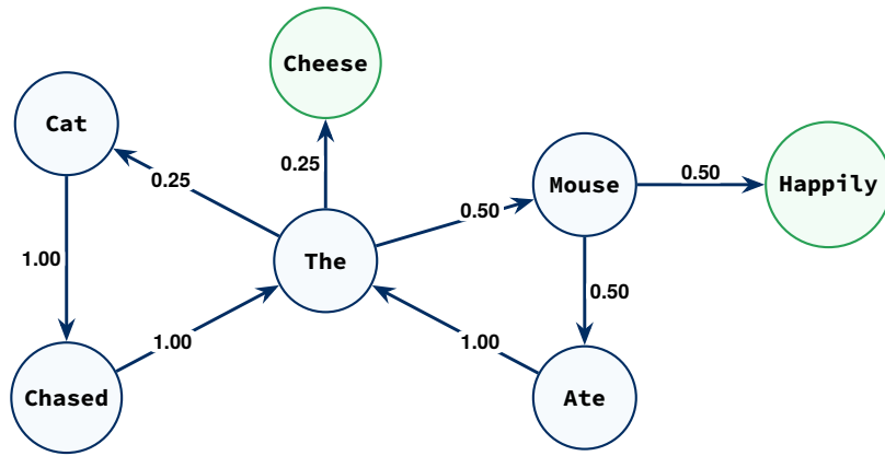
Figure 1.2: Markov state transition graph for the 7-token cat/mouse corpus. Directed edges indicate bigram transition probabilities \mathbb{P}(w_t \mid w_{t-1}) . States Cheese and Happily (green) are terminal absorbing states with zero outgoing probability mass.
