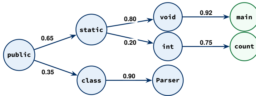
Figure 1.4: Markov chain state transition graph for software tokens.
