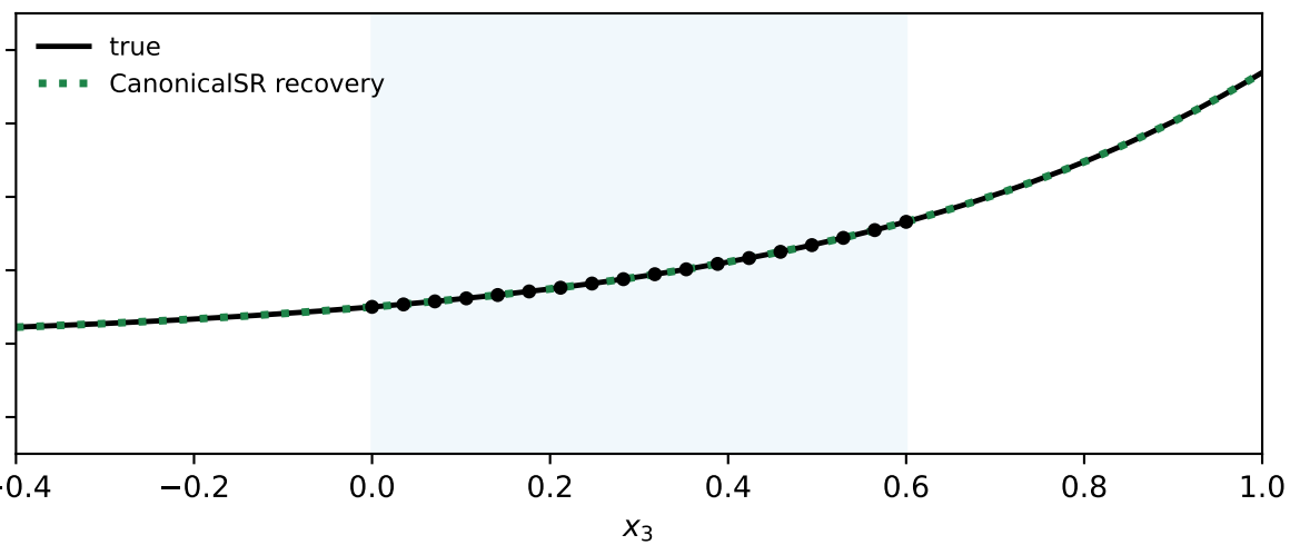
CANONICALSR — label-blind multi-route canonical recovery (near-exact fit first; among equally exact, fewest operators)
