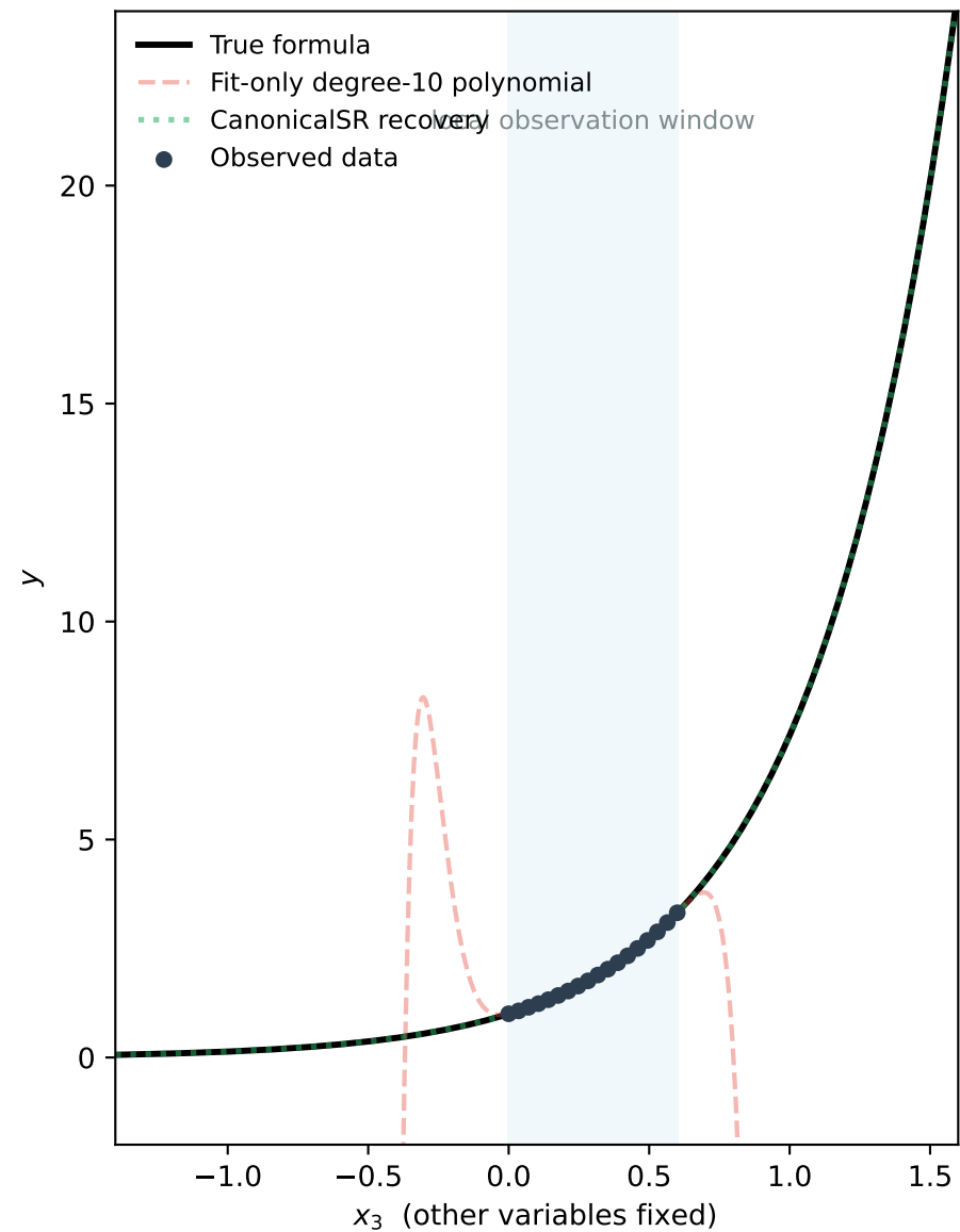
True formula, observed data, and both methods
