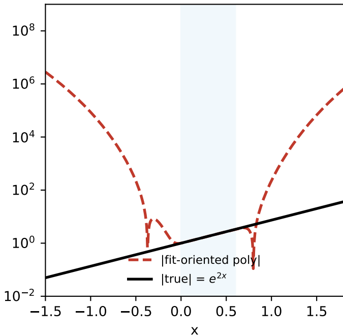
Extrapolation (log scale): decoration blows up
