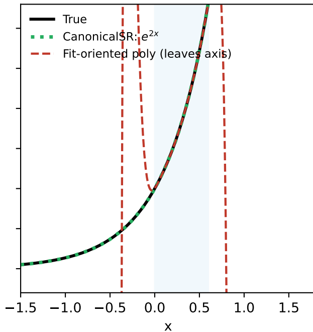
Extrapolation (zoom on true scale)
