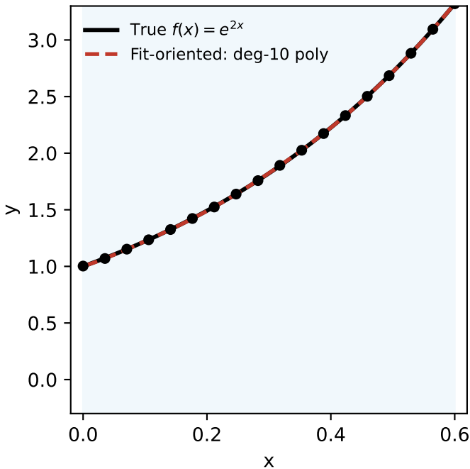
In-sample: both fit nearly perfectly (unidentifiable)
