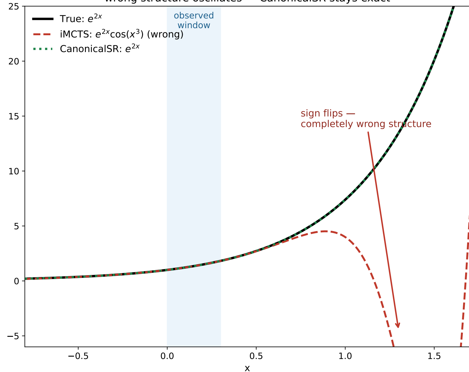
OUTSIDE the window: wrong structure oscillates — CanonicalSR stays exact
