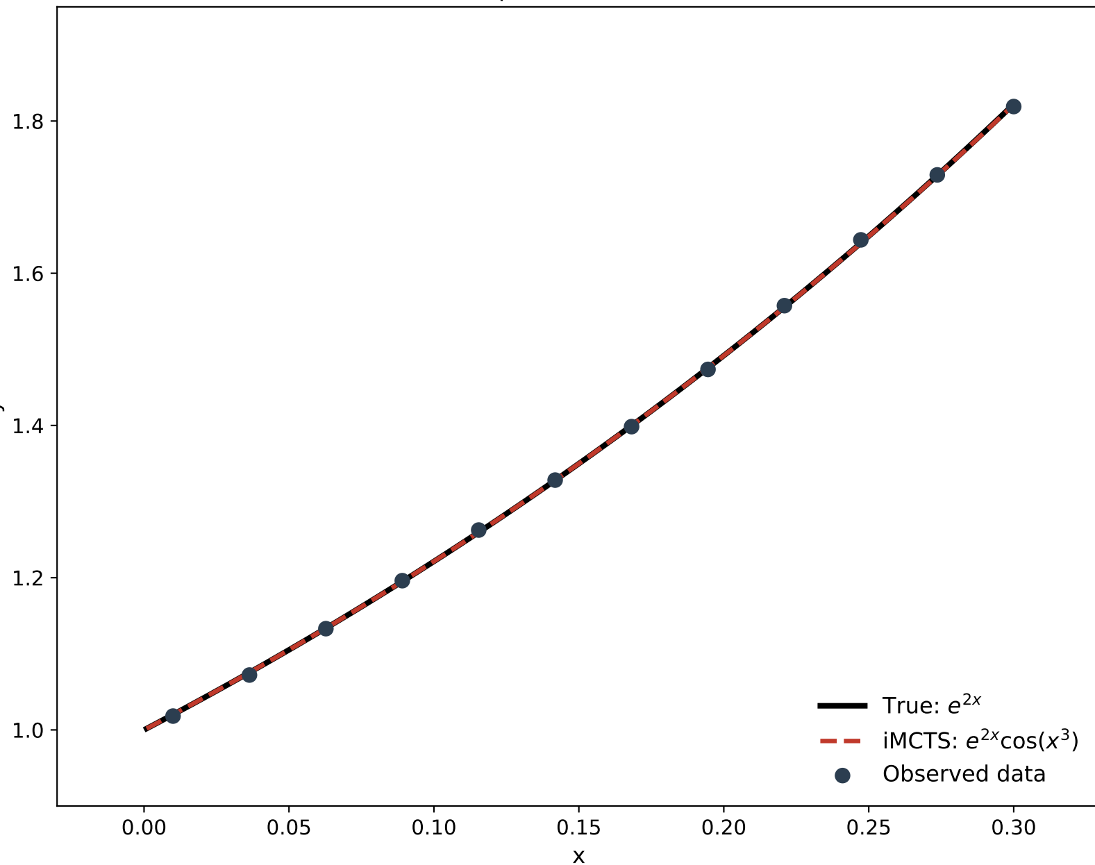
INSIDE the observation window: all curves overlap — structure not identifiable
