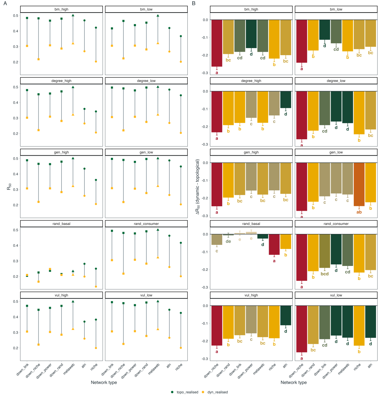
Figure 2: Differences between topological and dynamic estimates of network robustness. (A) Estimated robustness ( R_{50} ) of realised networks under topological (green) and dynamic (yellow) extinction simulations across network types and extinction scenarios. Points represent mean robustness values, with connecting lines highlighting the consistent reduction in robustness estimates when extinction cascades are evaluated dynamically. (B) Difference between dynamic and topological robustness estimates ( \Delta R_{50} = R_{50,dynamic} - R_{50,topological} ) for each network type. Negative values indicate that dynamic simulations produce lower inferred robustness than topological simulations. Bars show estimated marginal means from linear models accounting for differences among empirical communities; letters indicate significant differences among network types based on Sidak-adjusted pairwise comparisons.
