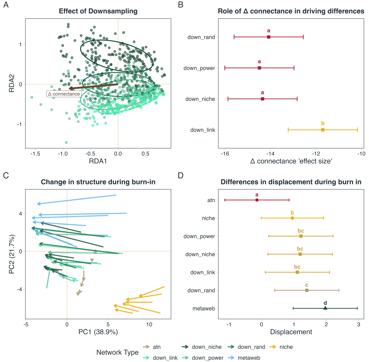
Figure 1: Downsampling approach influences both network topology and subsequent structural reorganisation during burn-in. (A) Redundancy analysis (RDA) ordination showing differences in network topology among downsampling approaches across the connectance gradient after accounting for community-level variation. (B) Estimated slopes ( \pm 95\% confidence intervals) describing the relationship between the primary RDA axis and connectance change for each downsampling approach; letters denote post-hoc groupings from estimated marginal trend comparisons. (C) Principal component trajectories illustrating structural change between network creation and burn-in for each downsampling approach. (D) Mean Euclidean displacement through PCA space during burn-in ( \pm 95\% confidence intervals); letters indicate pairwise differences among network types from estimated marginal means. Networks sharing the same letter are not significantly different.
