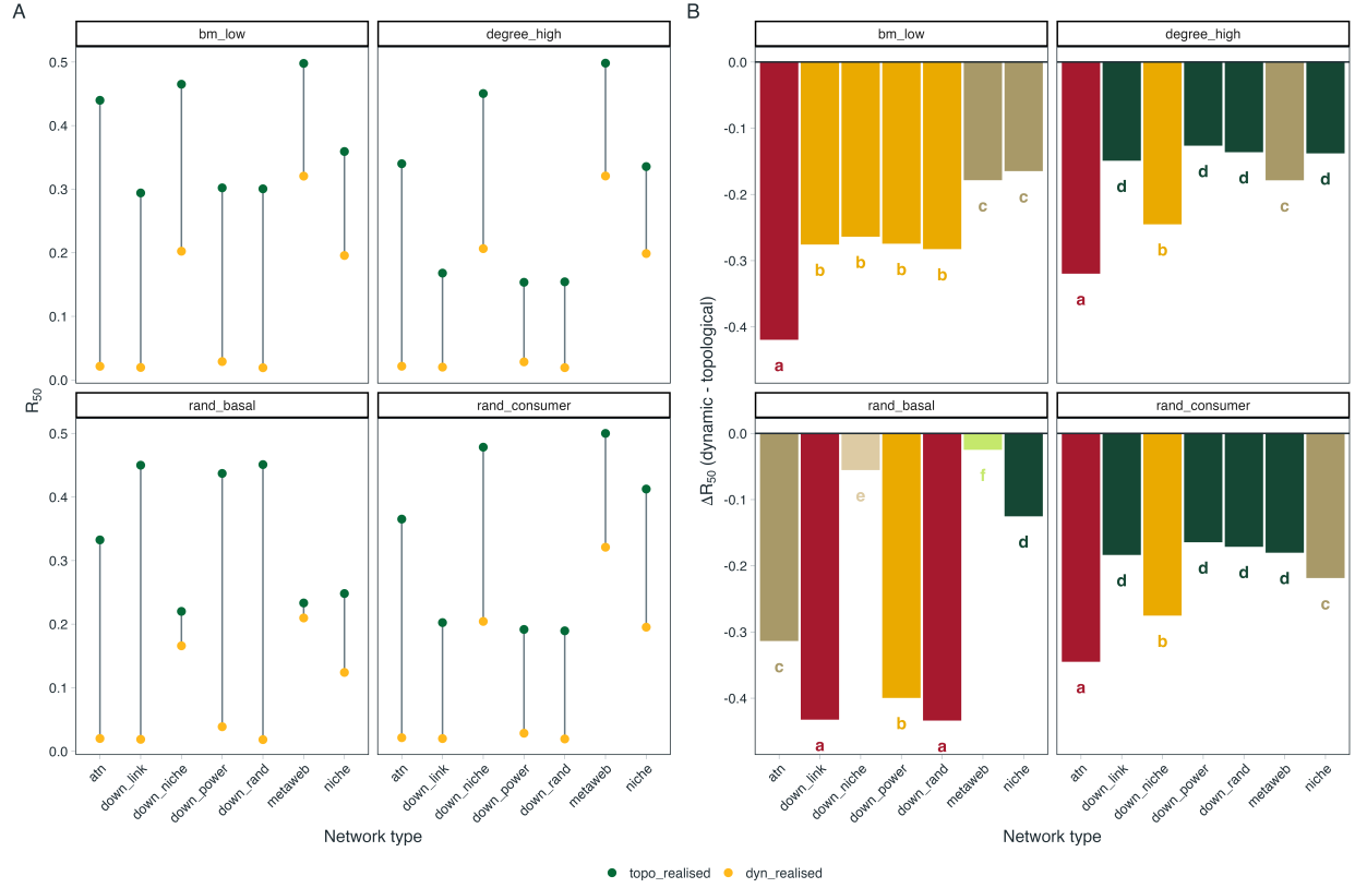
Figure 2: Differences between topological and dynamic estimates of network robustness. (A) Estimated robustness ( R_{50} ) of realised networks under topological (green) and dynamic (yellow) extinction simulations across network types and extinction scenarios. Points represent mean robustness values, with connecting lines highlighting the consistent reduction in robustness estimates when extinction cascades are evaluated dynamically. (B) Difference between dynamic and topological robustness estimates ( \Delta R_{50} = R_{50,dynamic} - R_{50,topological} ) for each network type. Negative values indicate that dynamic simulations produce lower inferred robustness than topological simulations. Bars show estimated marginal means from linear models accounting for differences among empirical communities; letters indicate significant differences among network types based on Sidak-adjusted pairwise comparisons.
