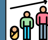
Average of Charges by BMI Bracket and Smoker Status
