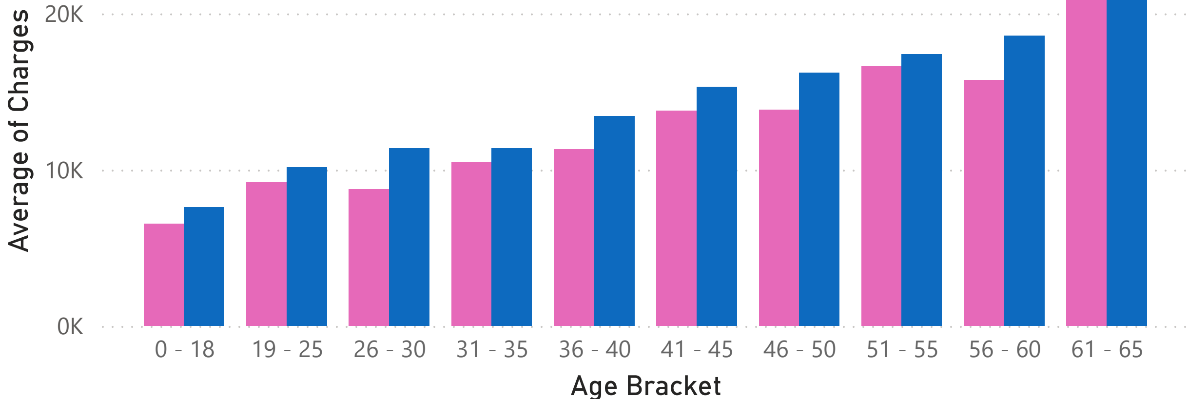
Average of Charges by Age Bracket and Children
