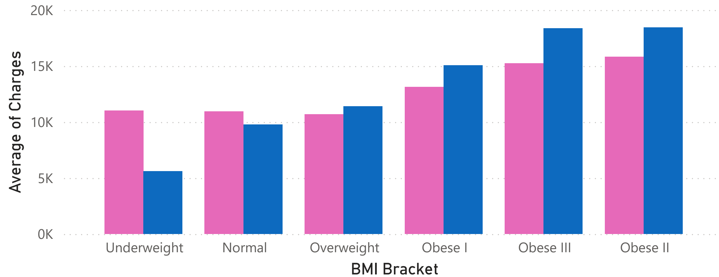
Average of Charges by BMI Bracket and Children
