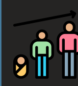
Average of Charges by Age Bracket and Smoker Status
