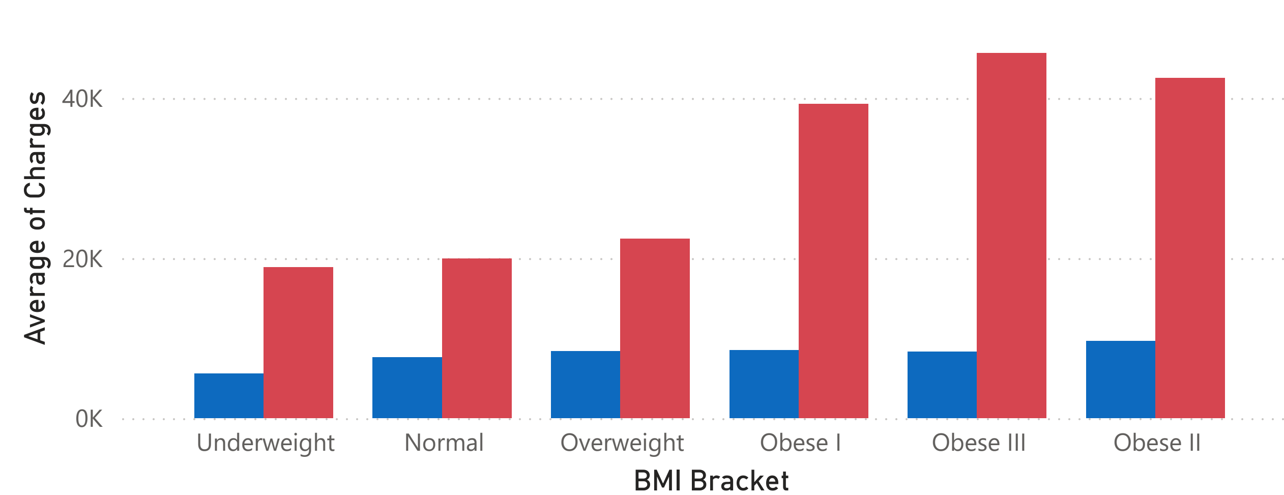
Average of Charges by BMI Bracket and Region
