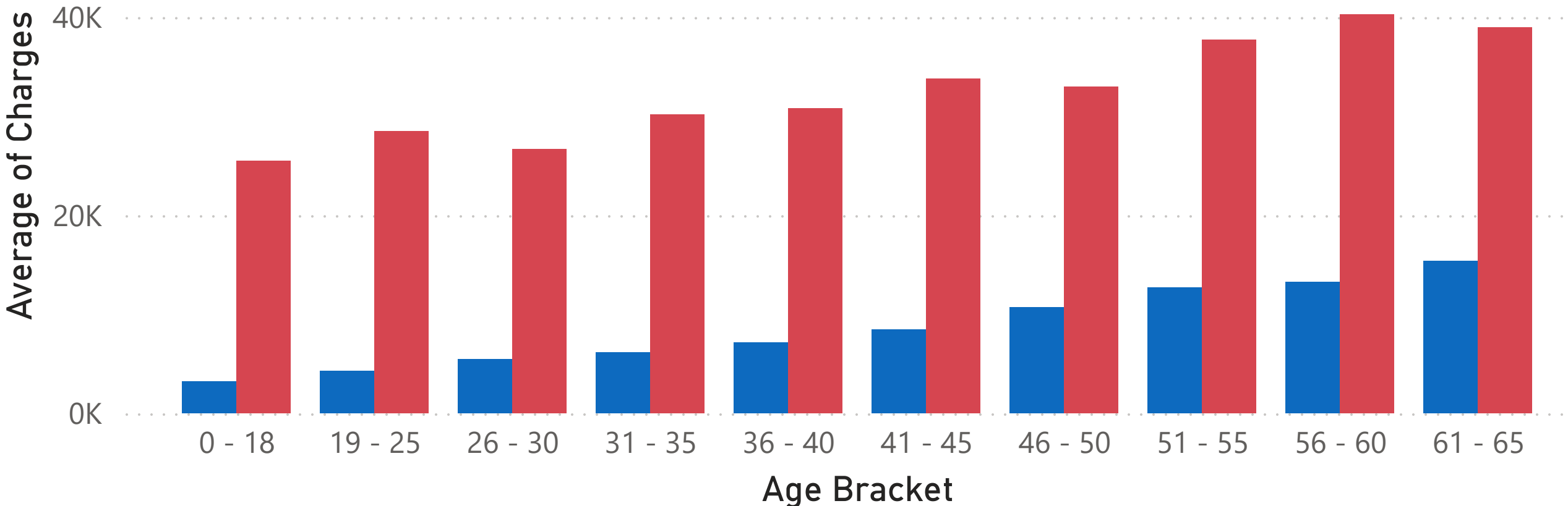
Average of Charges by Age Bracket and Region
