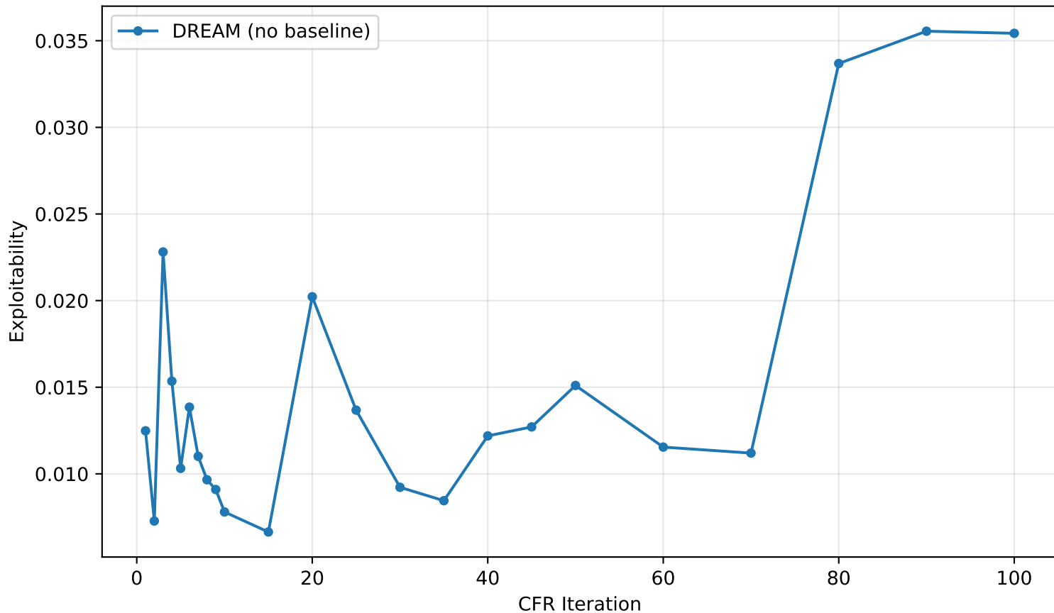
2x2 CDH Dark Hex: DREAM Convergence
