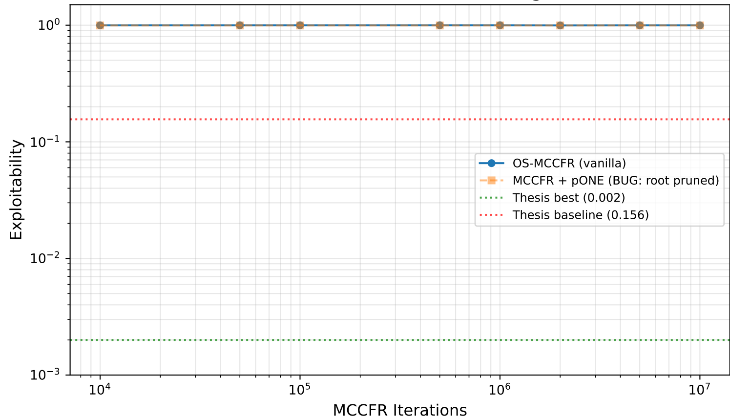
4x3 CDH Dark Hex: MCCFR Convergence
