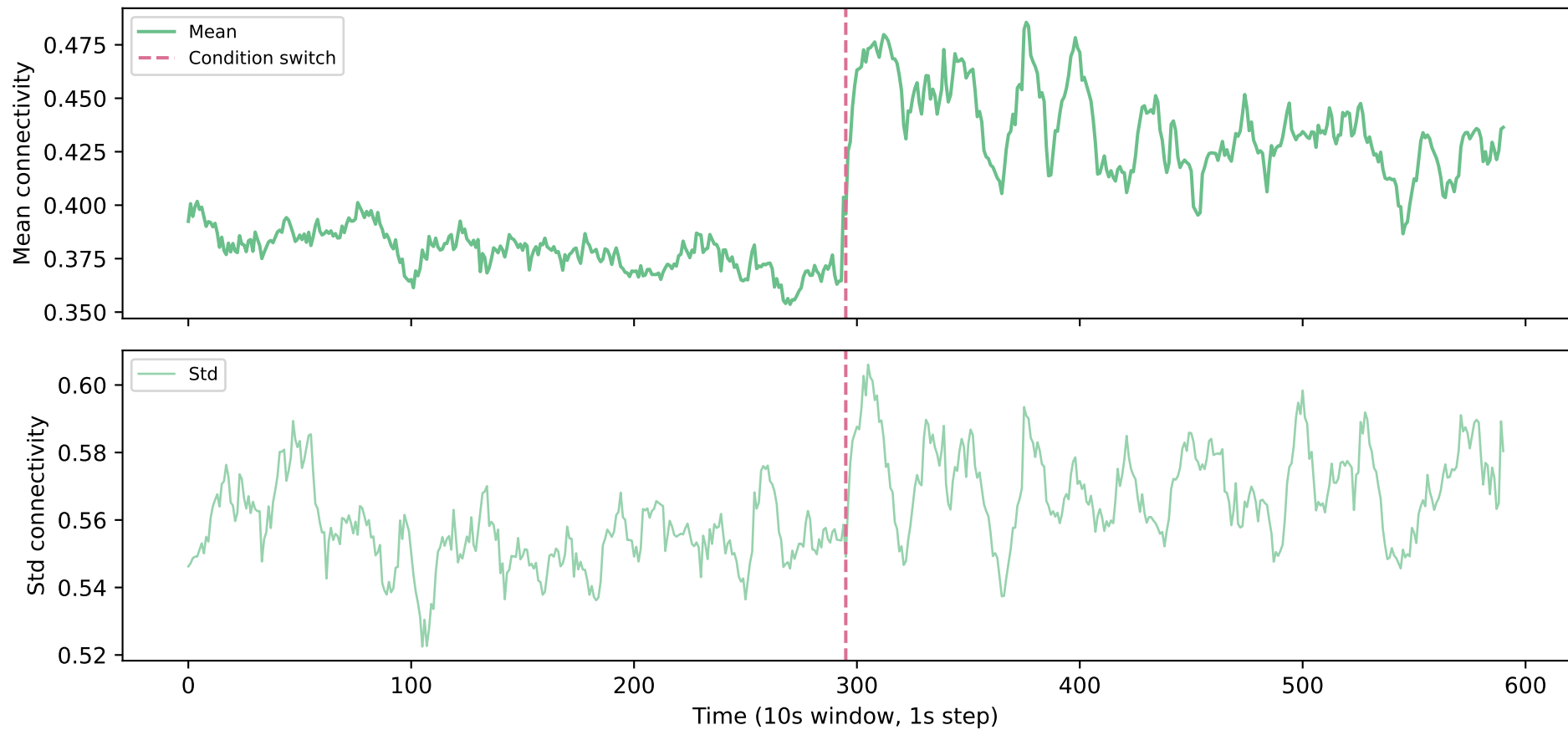
C01 — Central <-> Central
