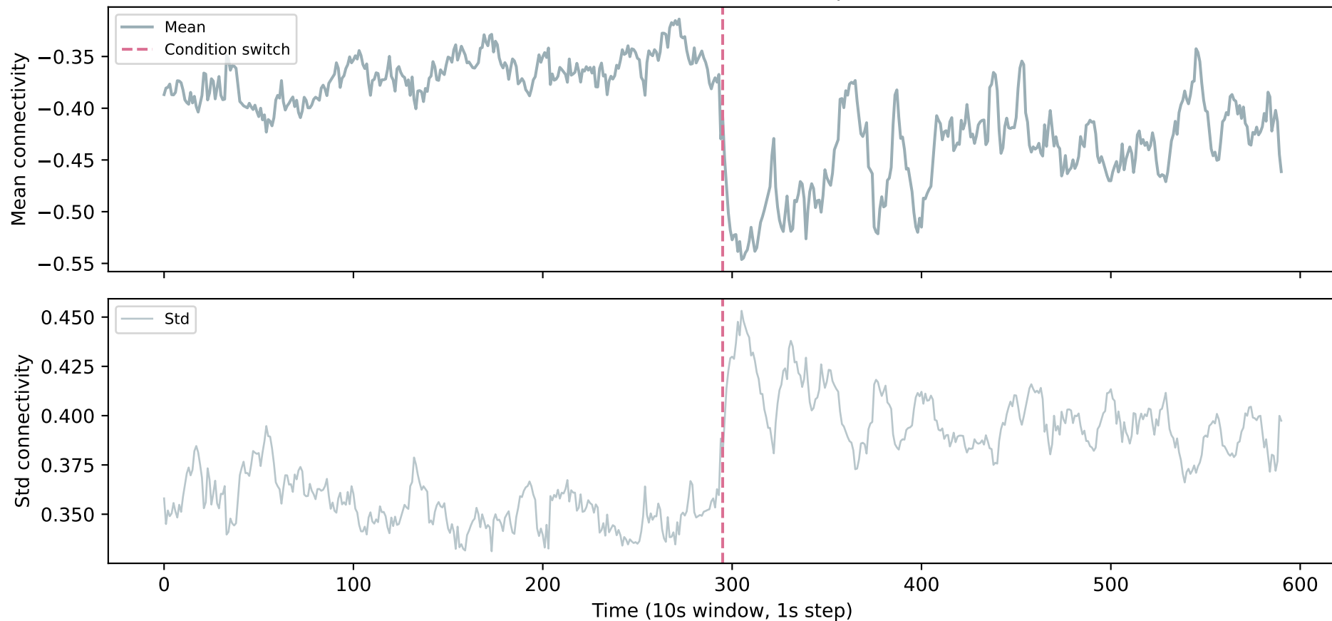
C01 — Central <-> Occipital
