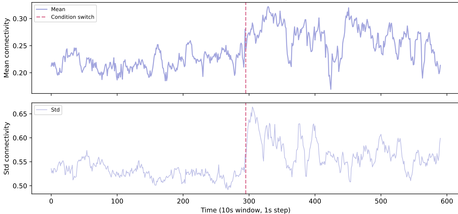
C01 — Parietal <-> Occipital
