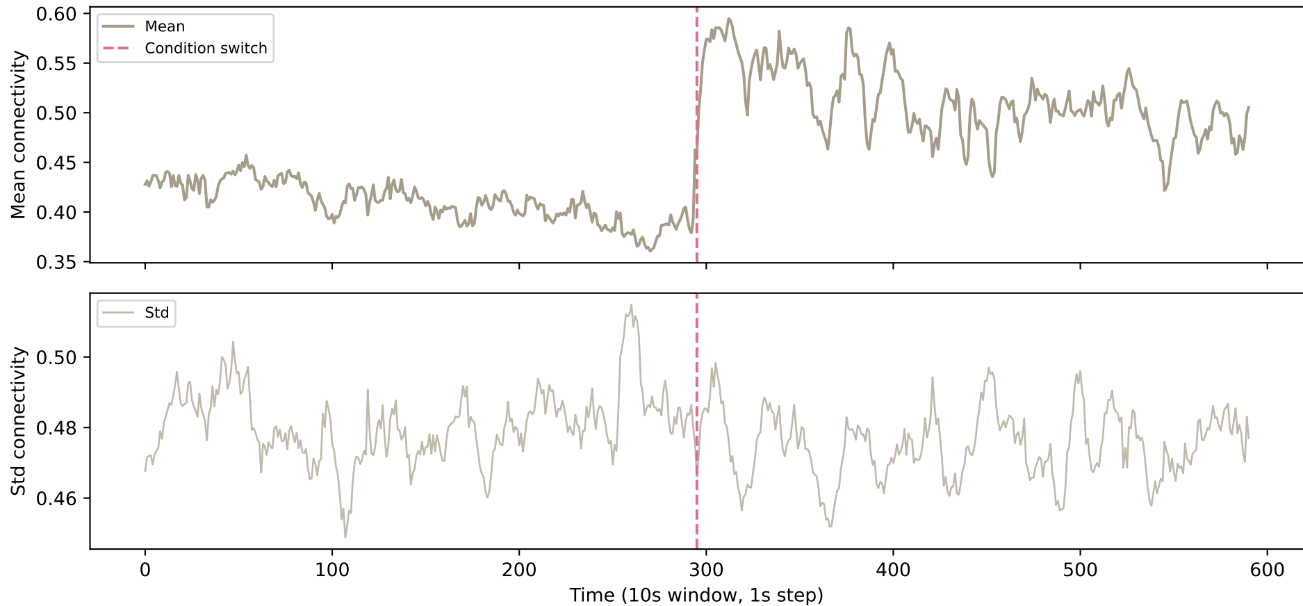
C01 — Frontal <-> Central
