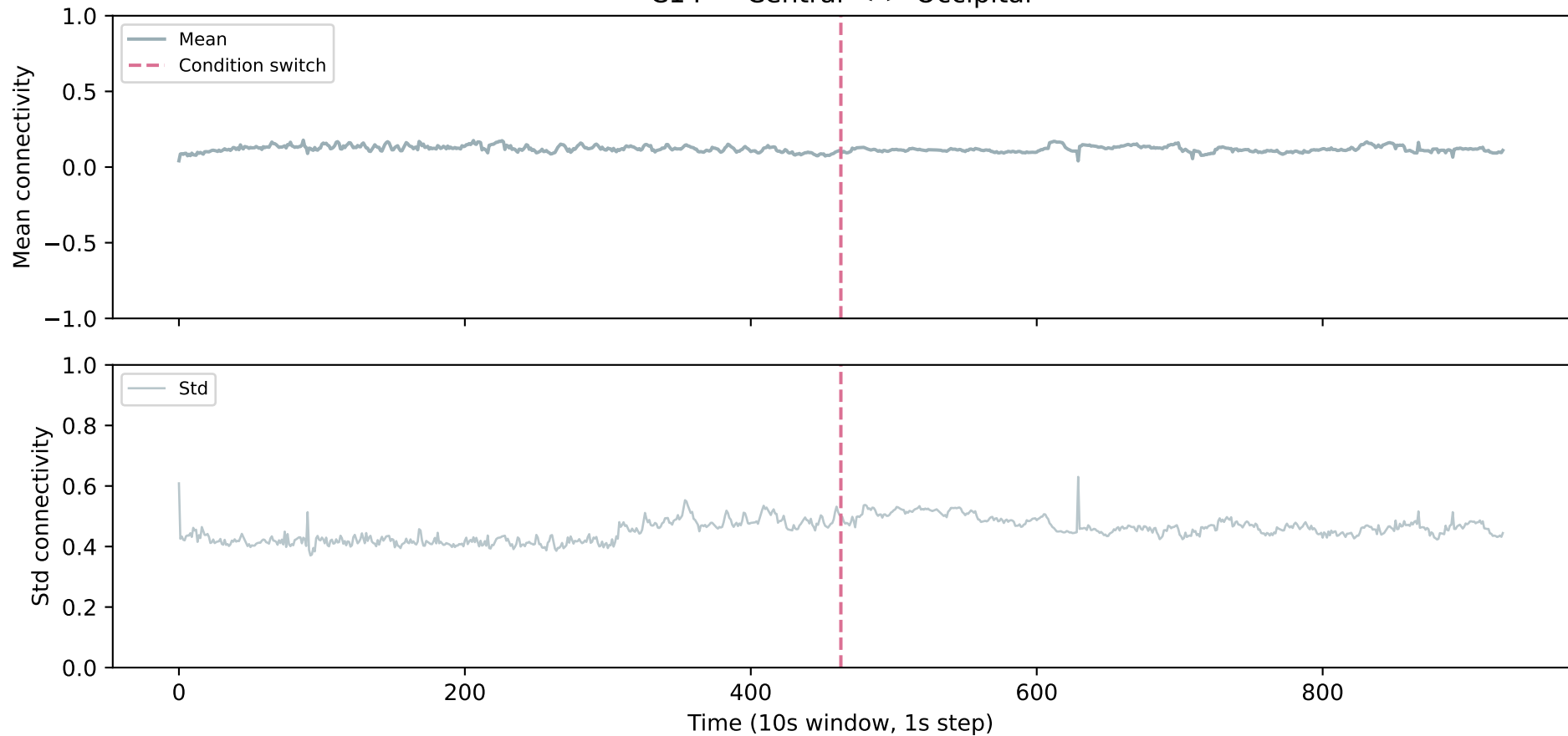
C14 — Central <-> Occipital
