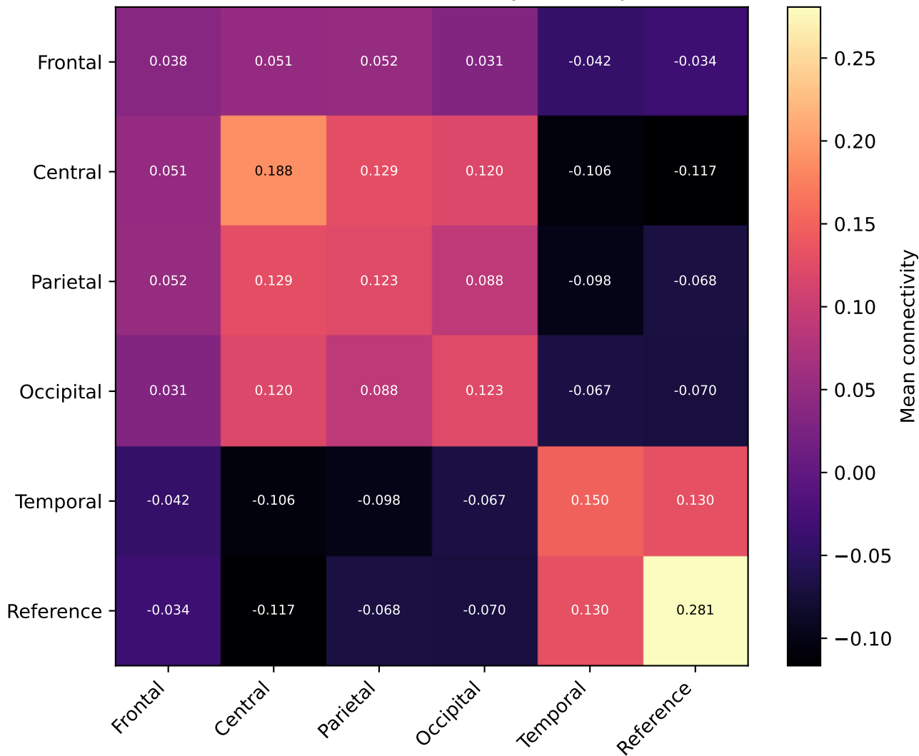
C14 — mean connectivity heatmap
