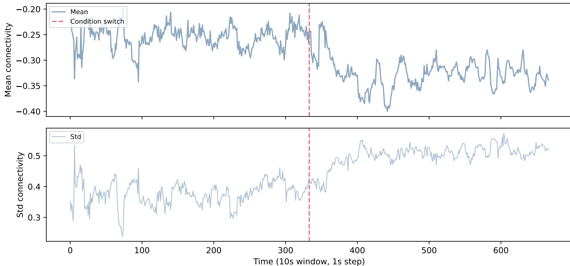
C22 — Parietal <-> Reference
