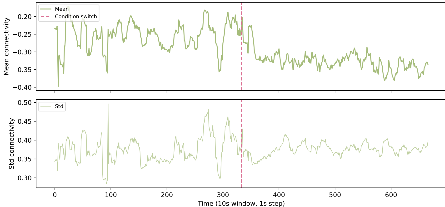
C22 — Central <-> Temporal
