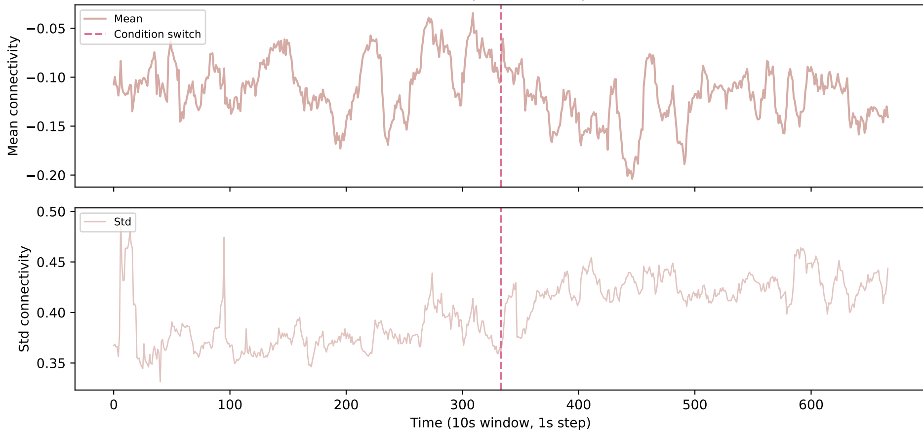
C22 — Occipital <-> Temporal
