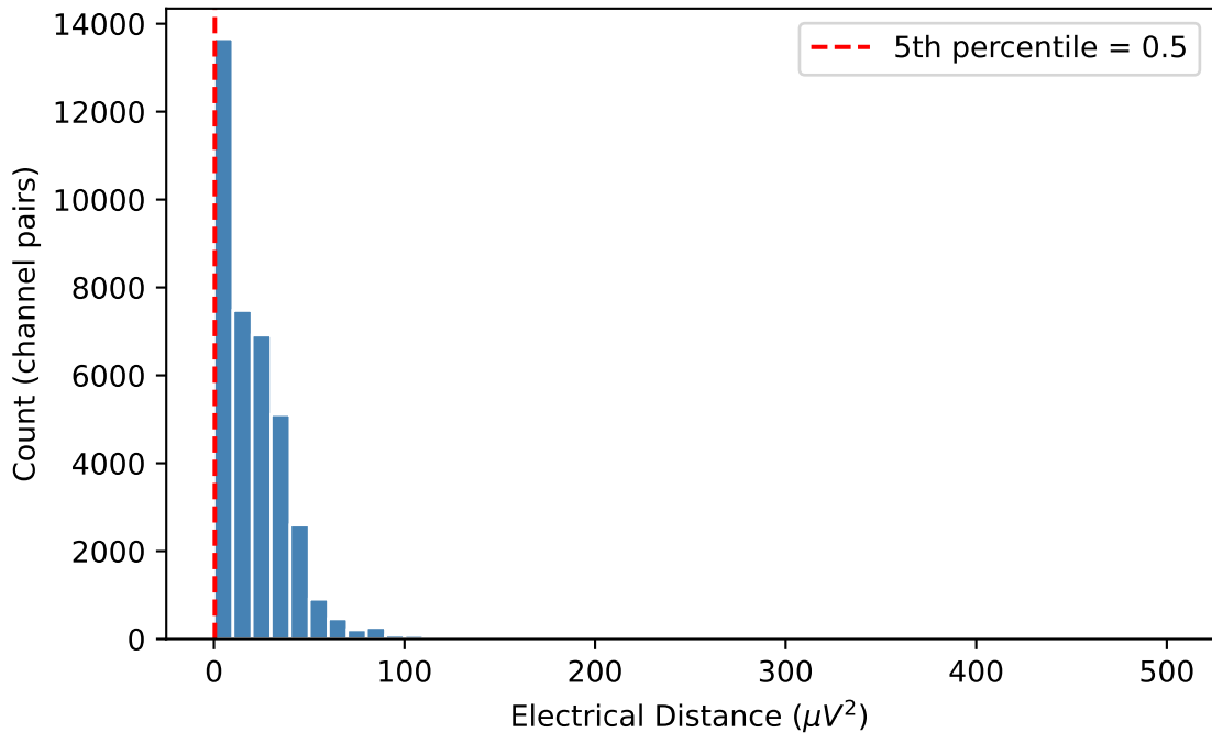
Electrical Distance Distribution — C01
