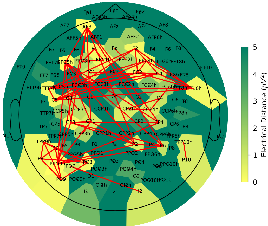
Bridged Electrodes — C02 | 60s | 100Hz
