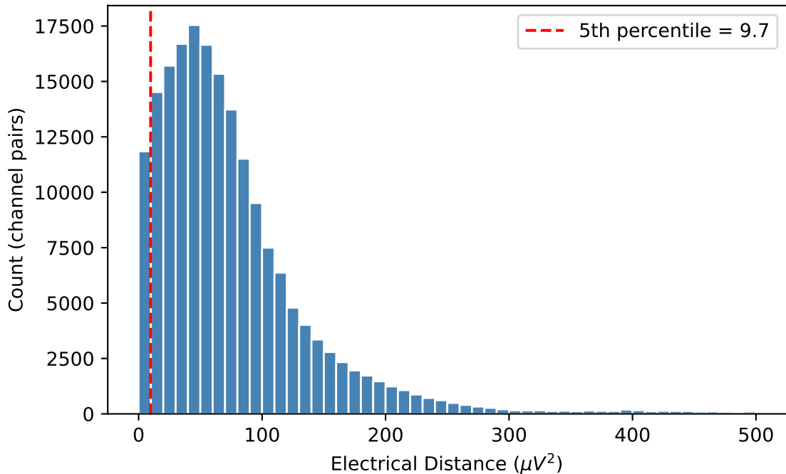
Electrical Distance Distribution — C02
