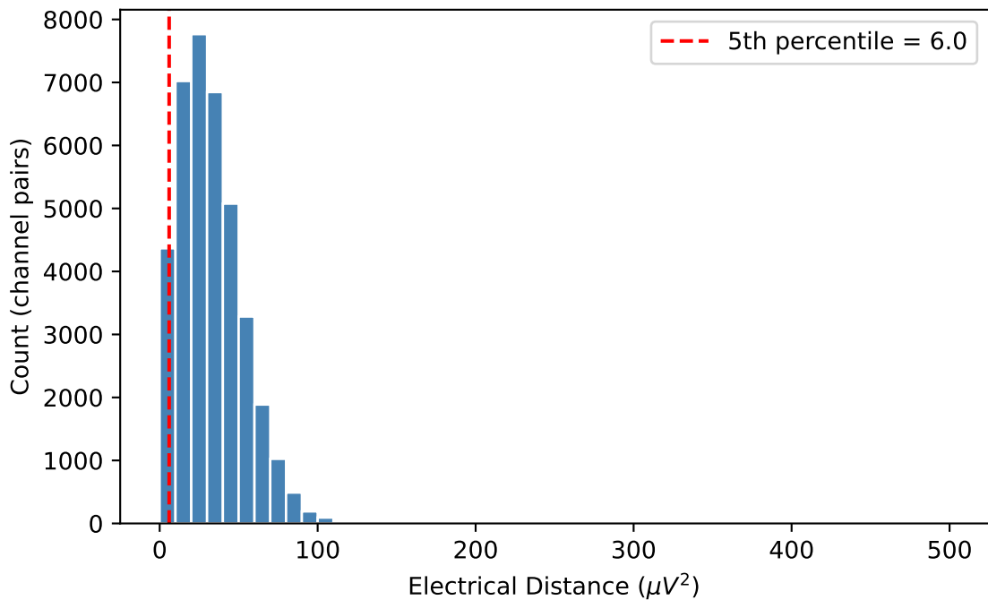
Electrical Distance Distribution — C05
