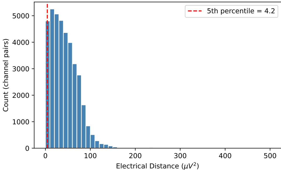
Electrical Distance Distribution — C07
