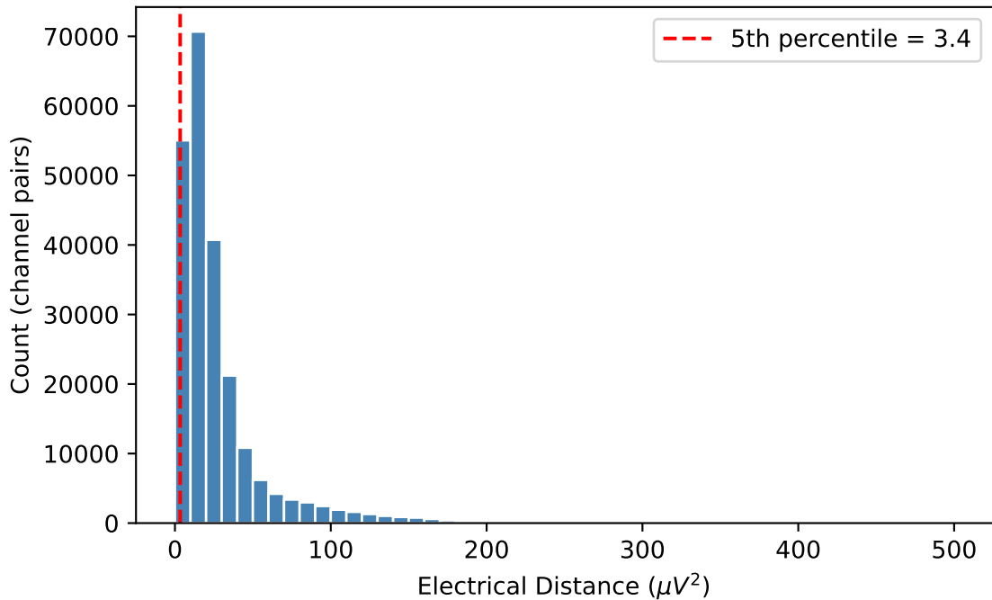
Electrical Distance Distribution — C08
