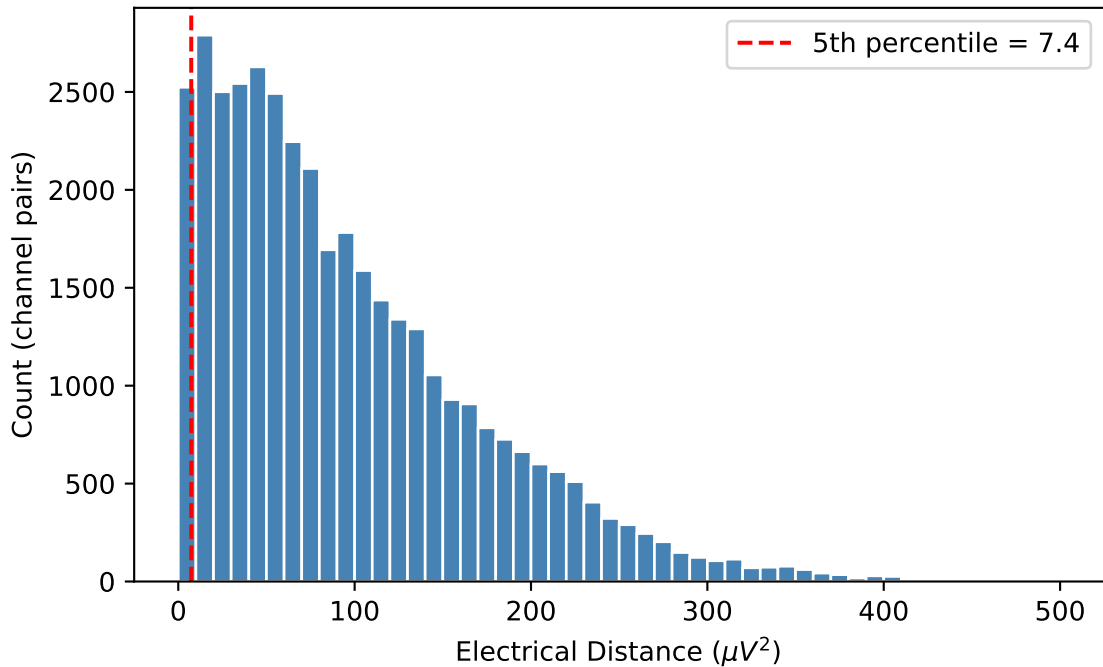
Electrical Distance Distribution — C10
