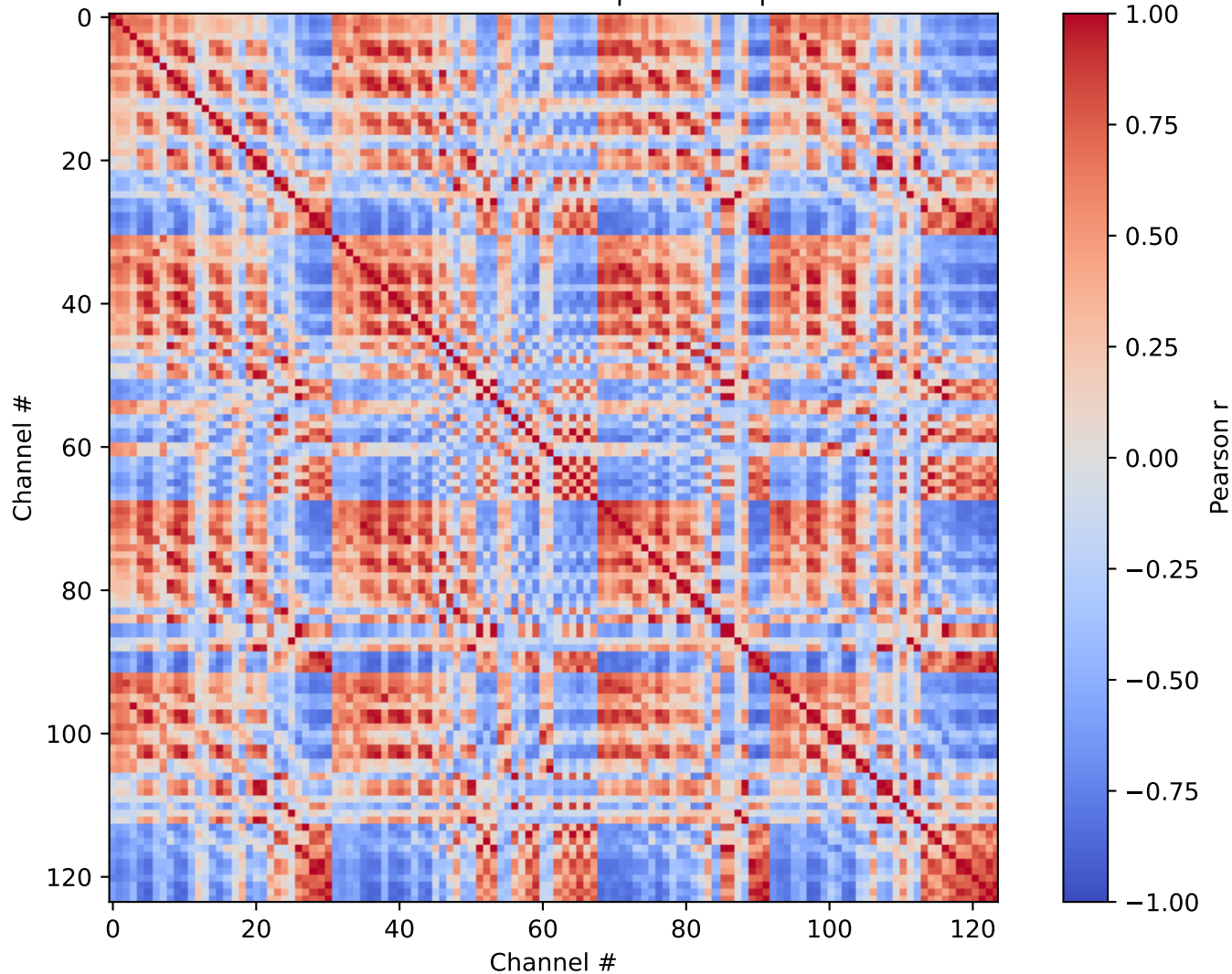
Correlation Matrix — C10 | last 10s | 100Hz
