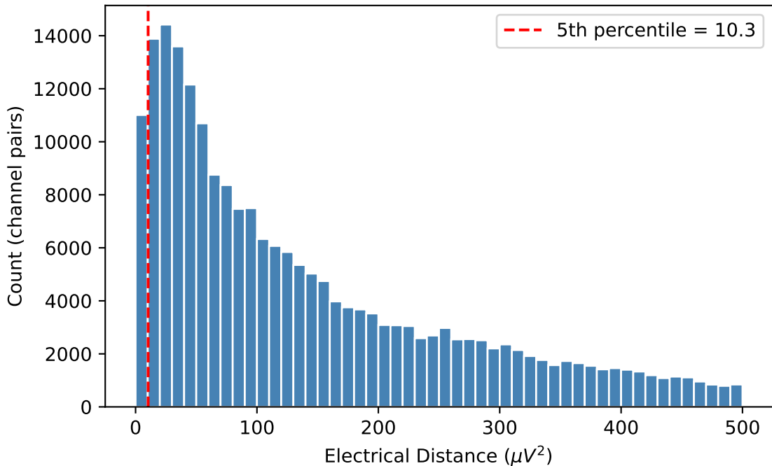
Electrical Distance Distribution — C11
