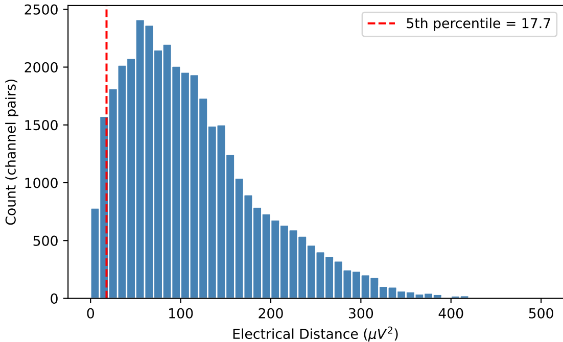
Electrical Distance Distribution — C12
