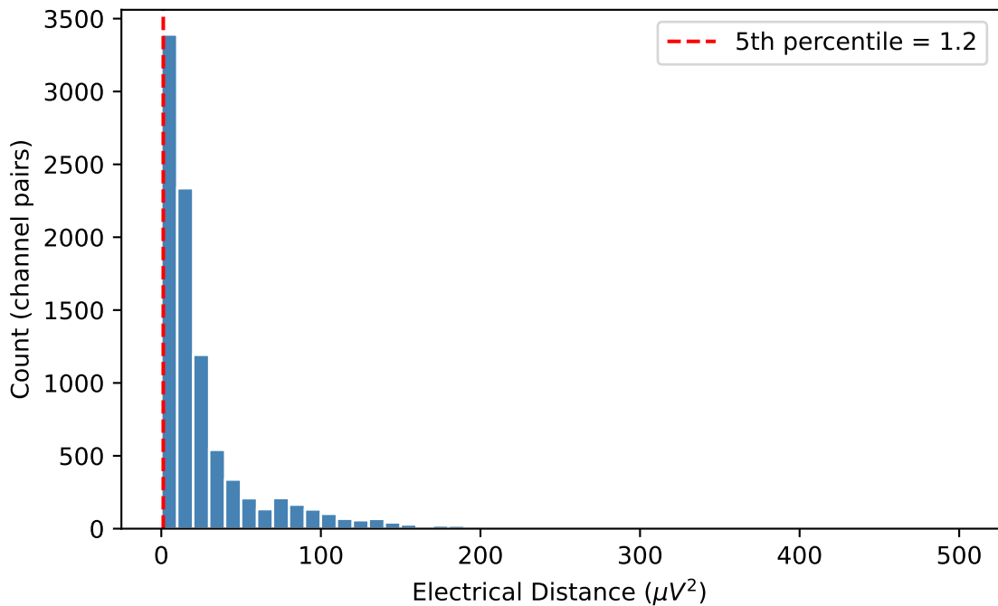
Electrical Distance Distribution — C14
