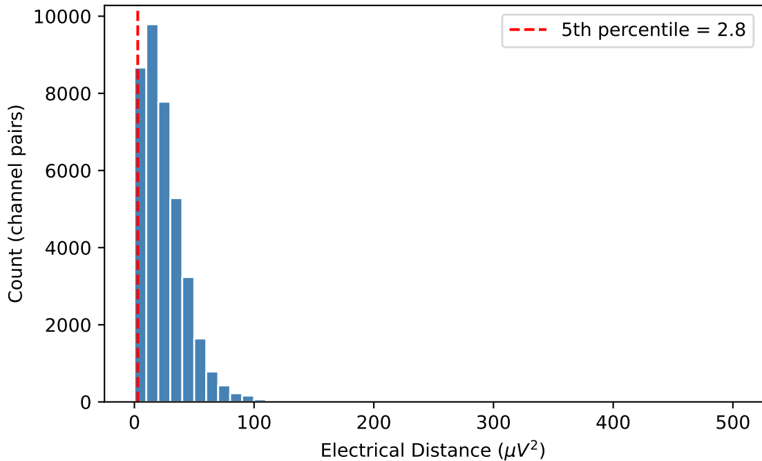
Electrical Distance Distribution — C18
