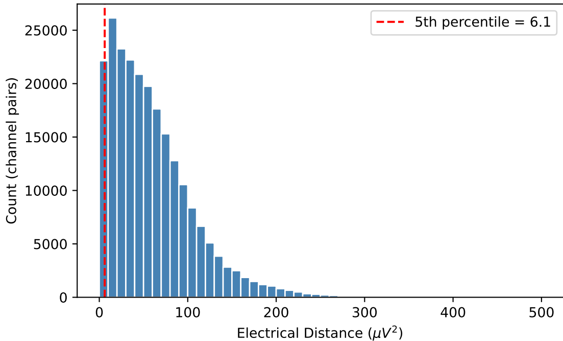
Electrical Distance Distribution — C19
