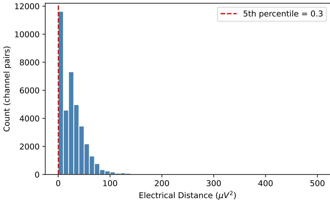
Electrical Distance Distribution — C24
