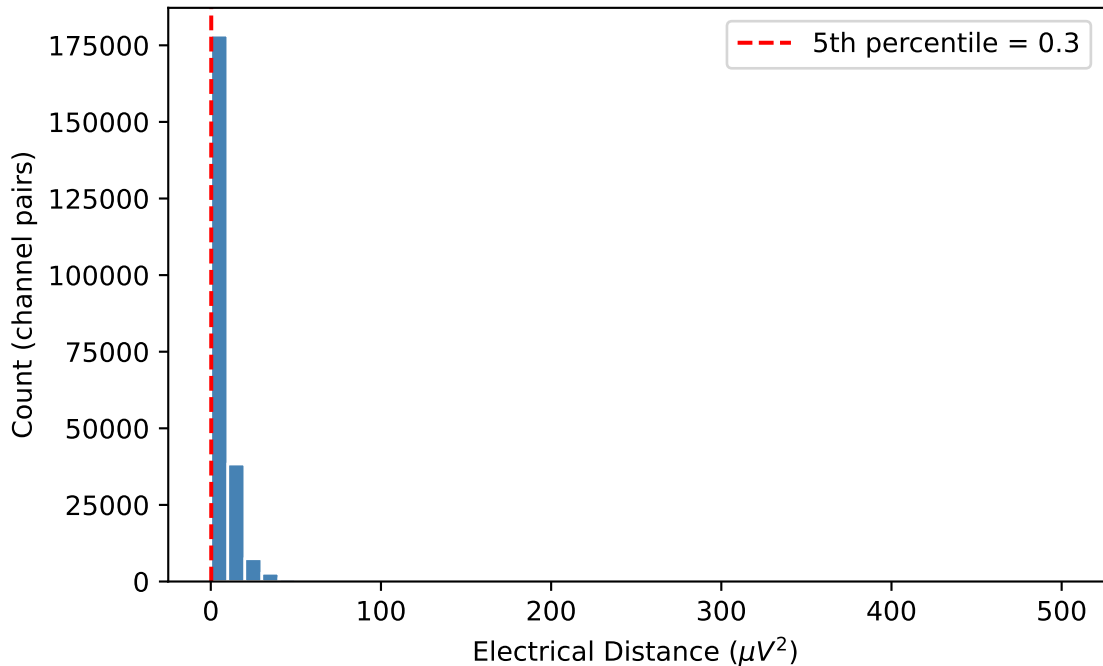
Electrical Distance Distribution — C26
