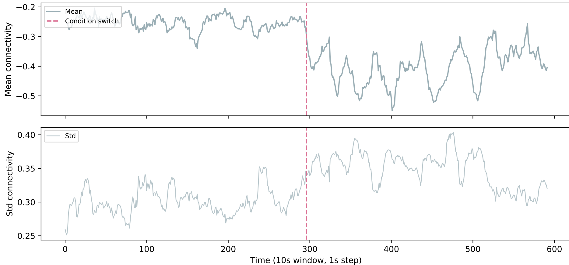
C03 — Central <-> Occipital
