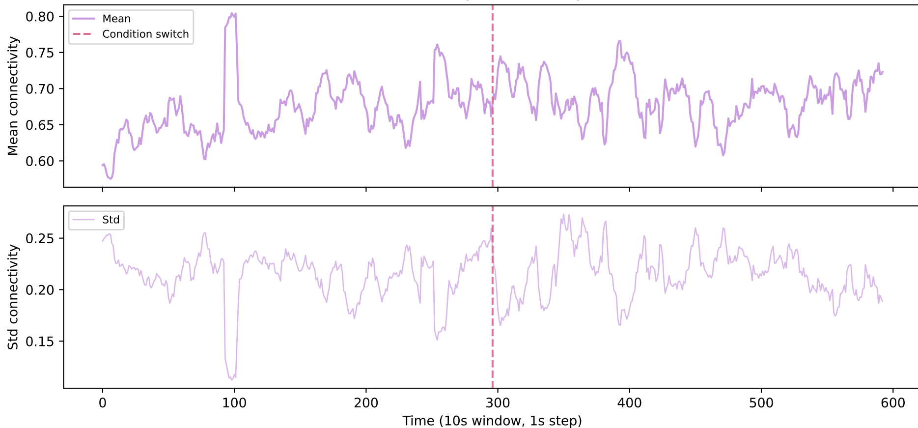
C05 — Occipital <-> Occipital
