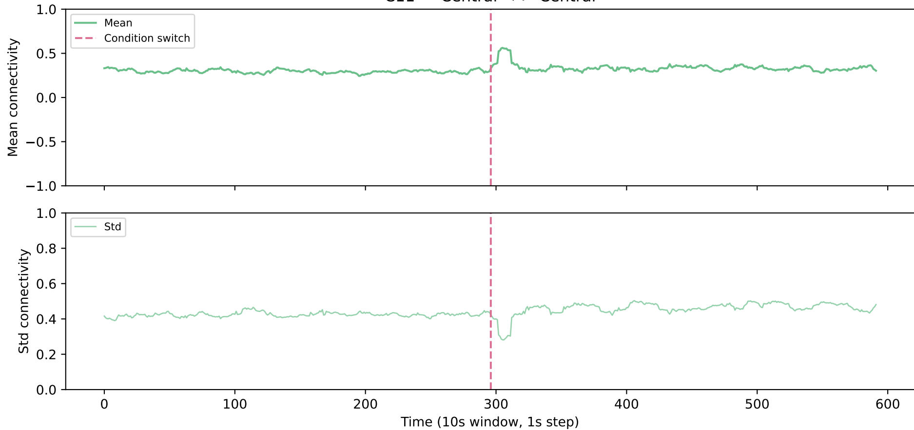
C11 — Central <-> Central
