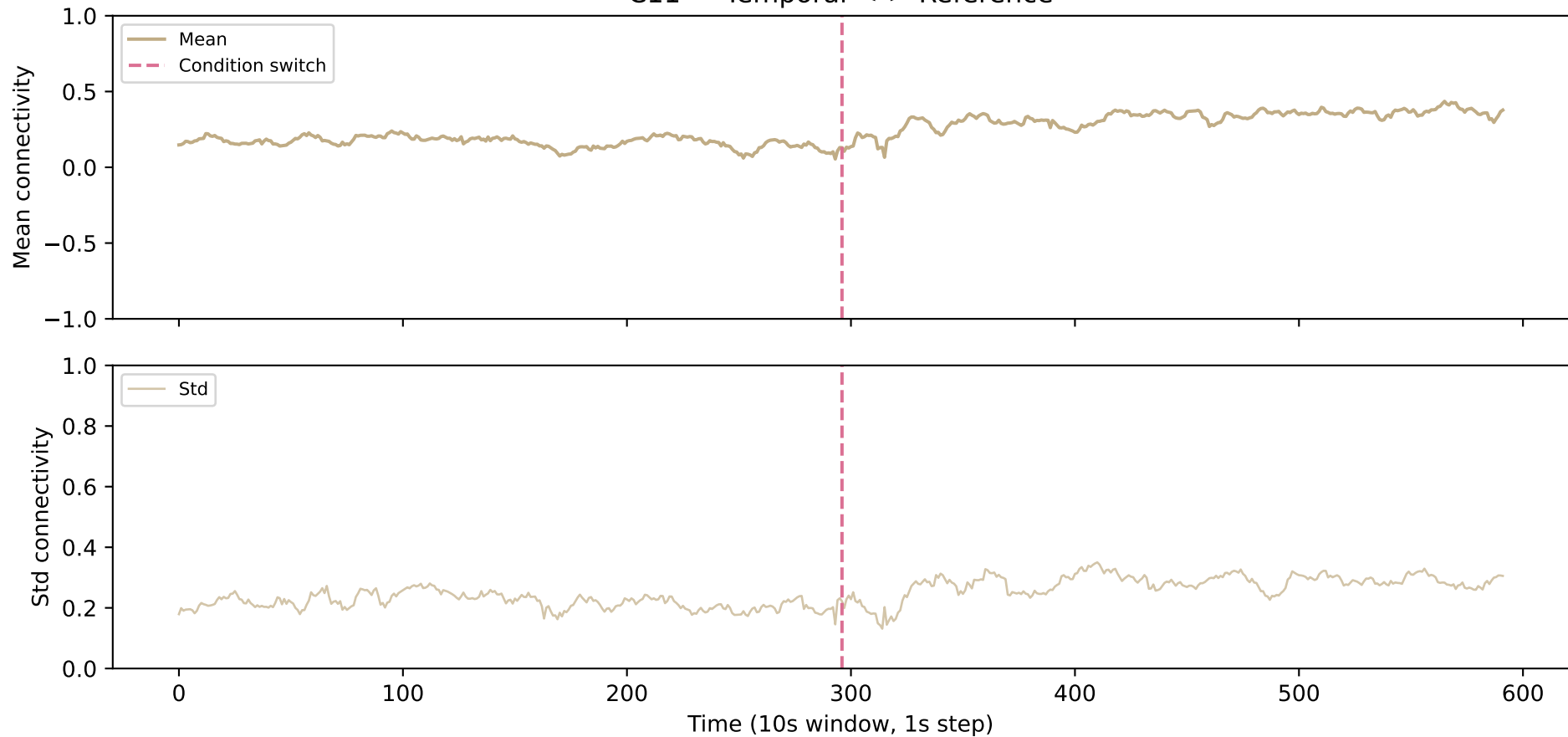
C11 — Temporal <-> Reference
