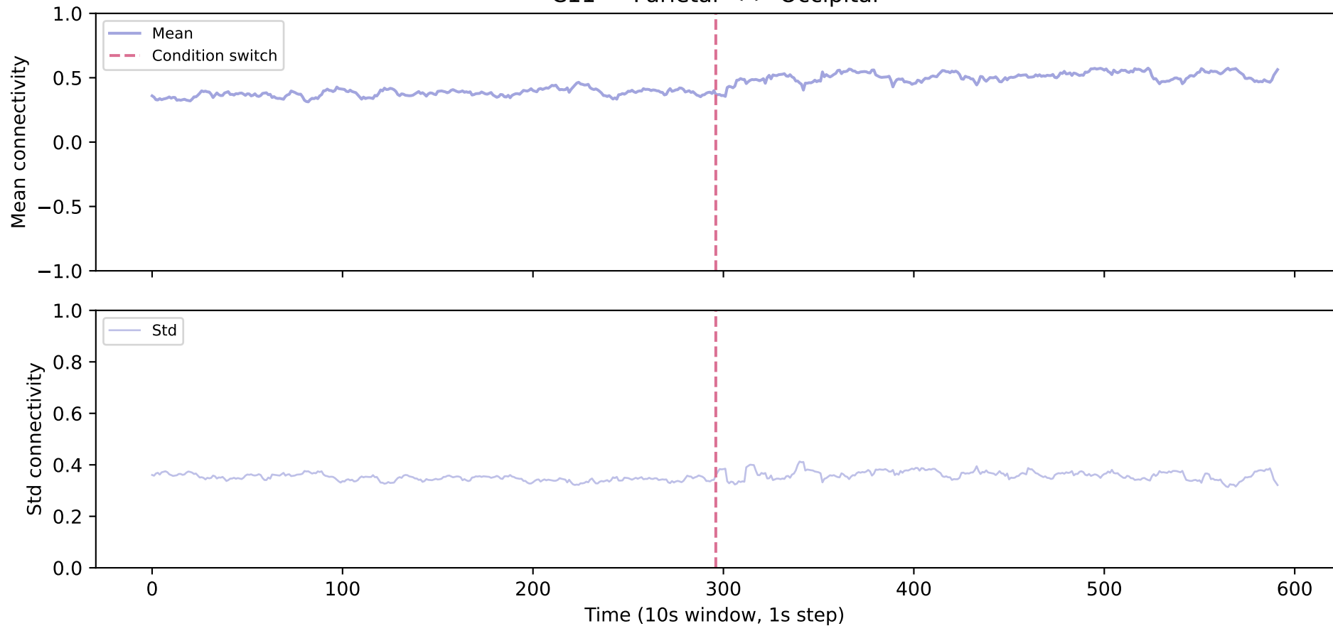
C11 — Parietal <-> Occipital
