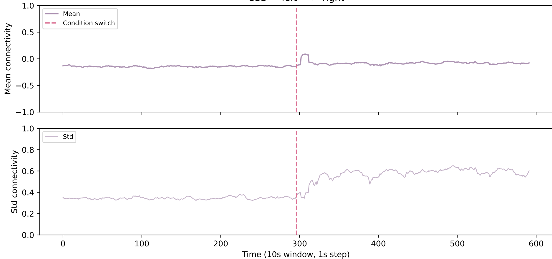
C11 — left <-> right
