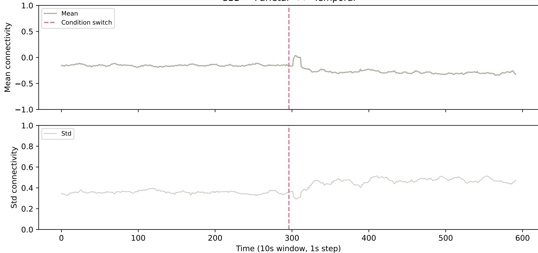
C11 — Parietal <-> Temporal
