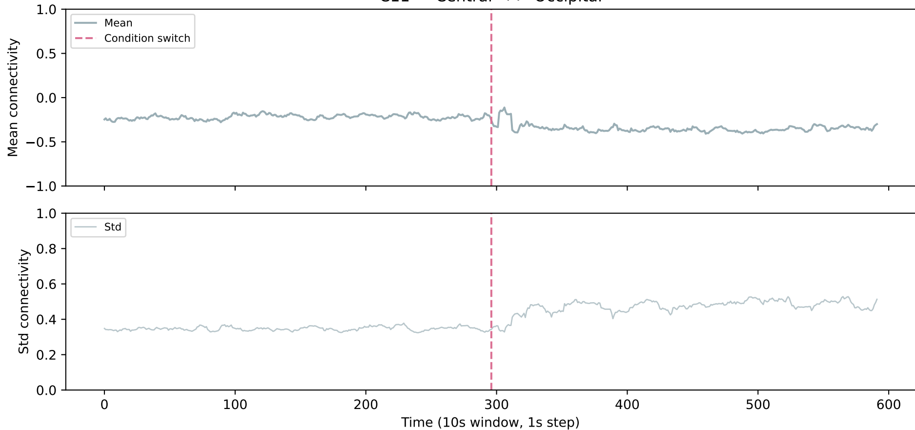
C11 — Central <-> Occipital
