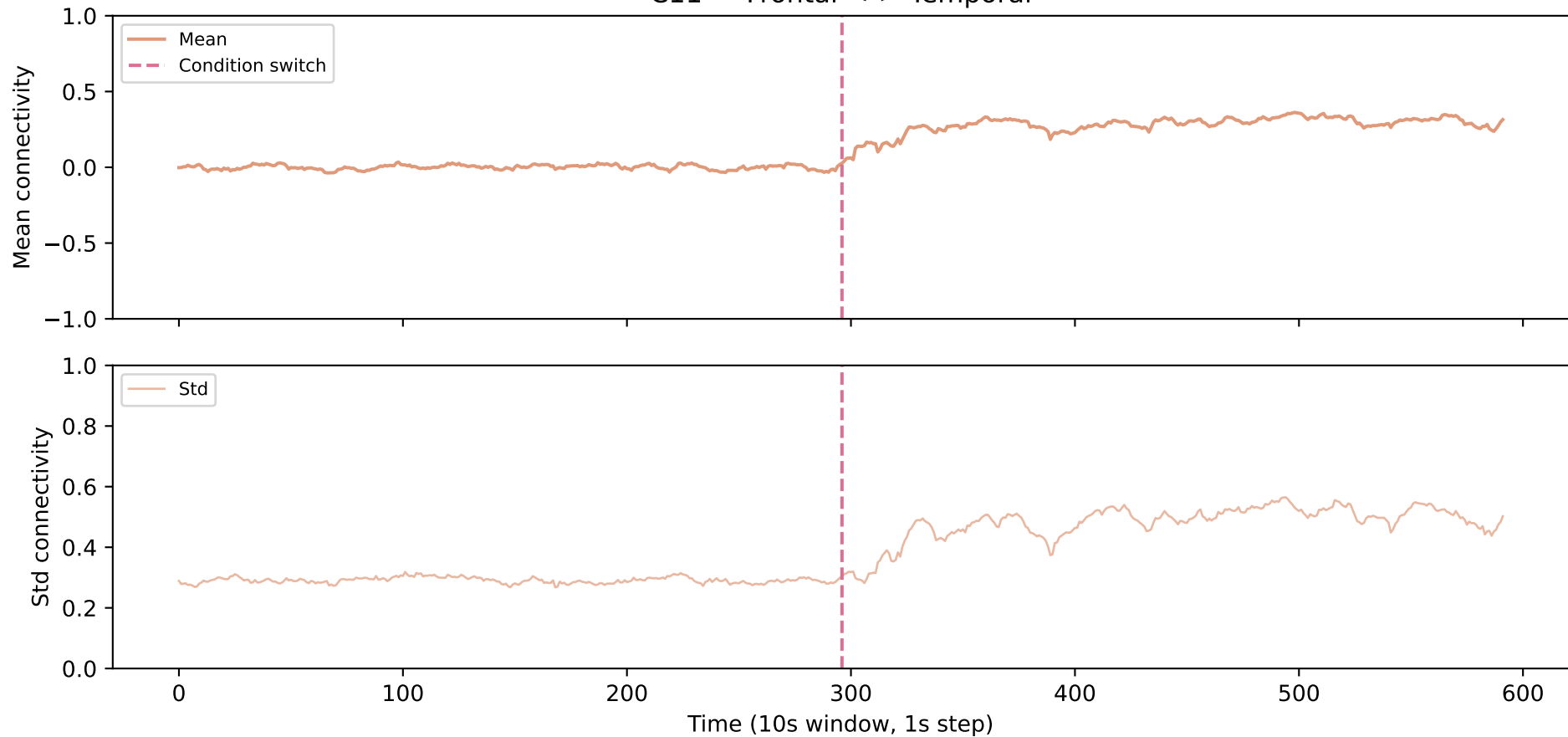
C11 — Frontal <-> Temporal
