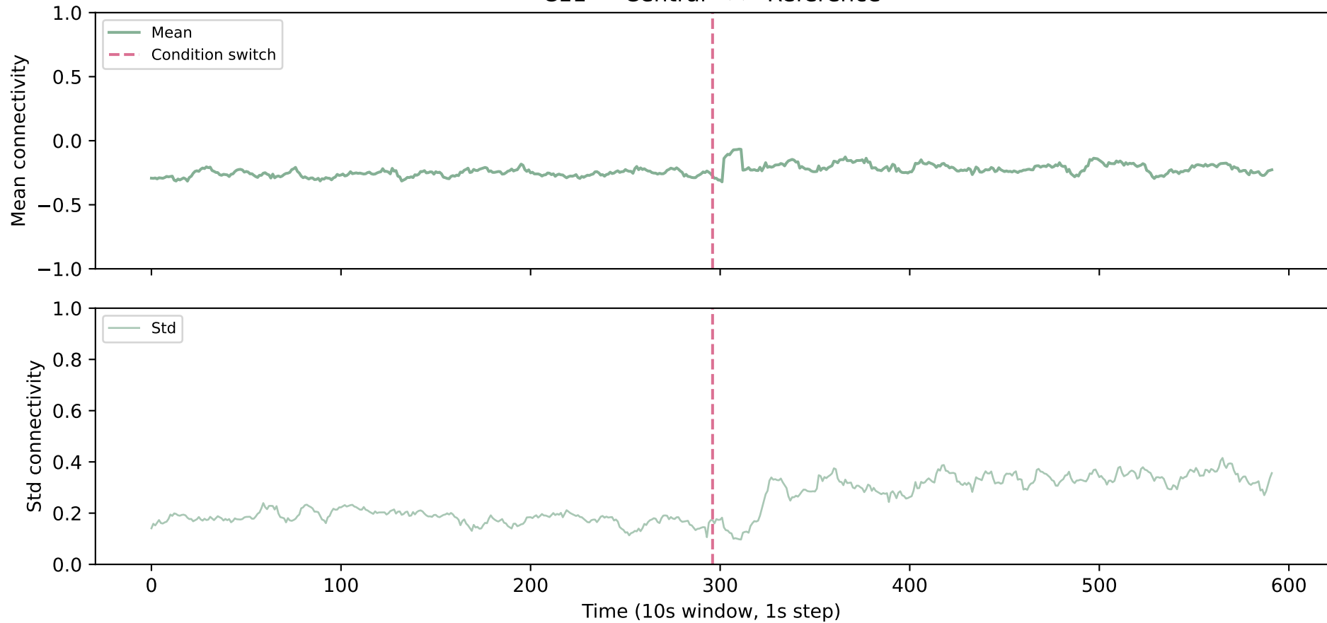
C11 — Central <-> Reference
