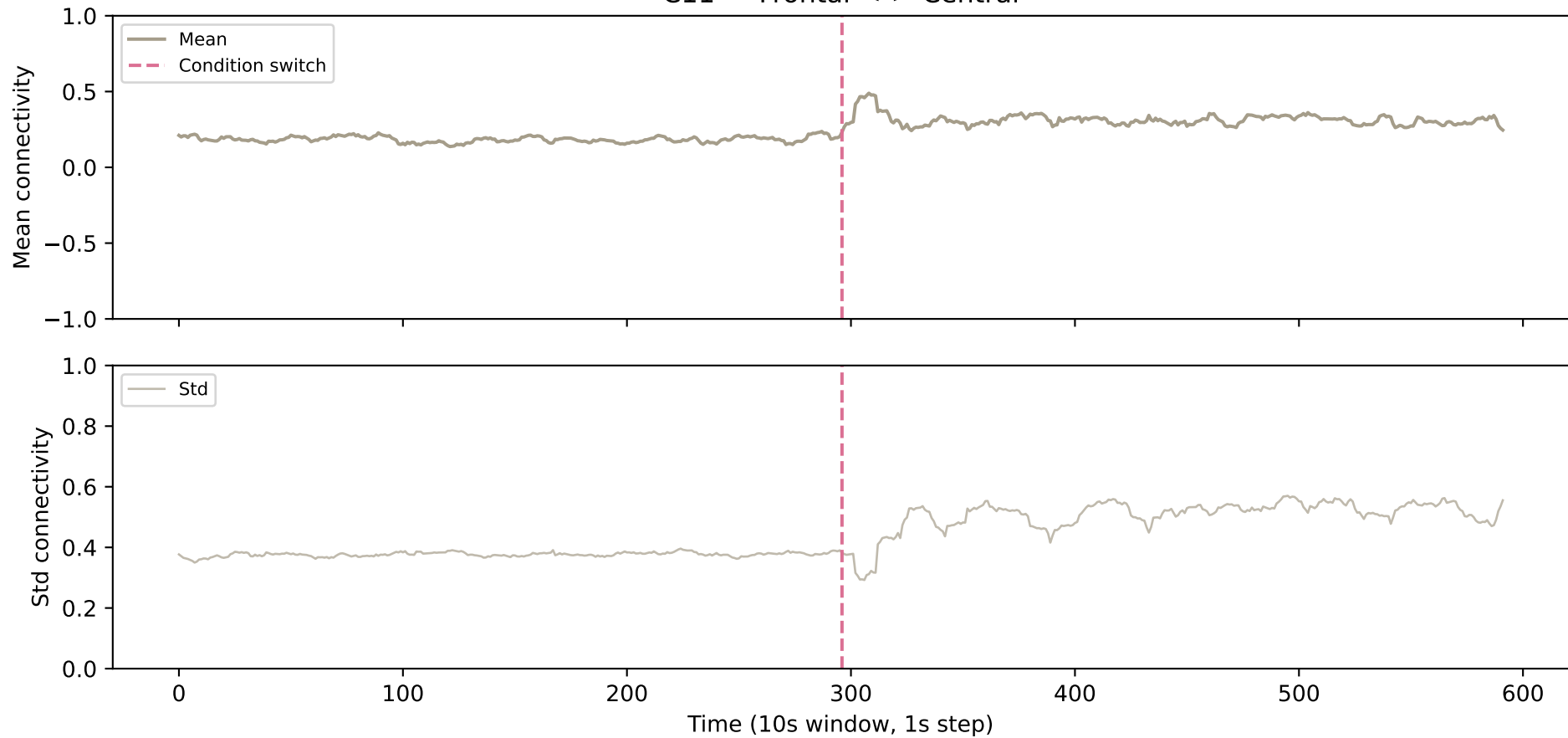
C11 — Frontal <-> Central
