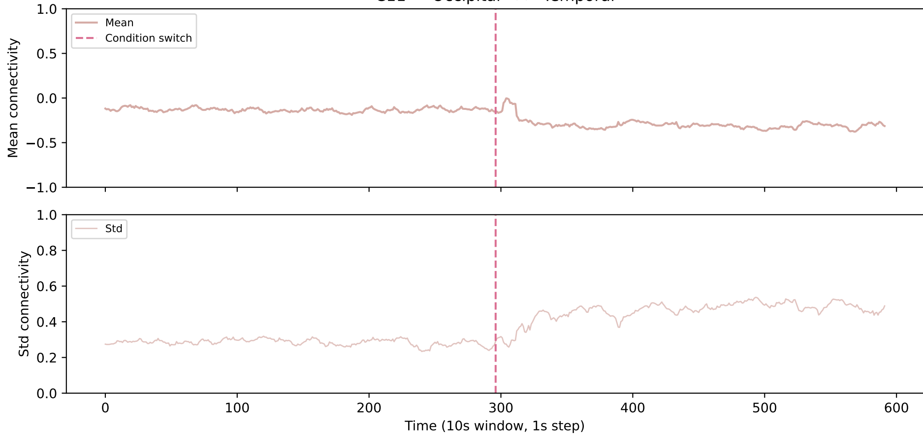
C11 — Occipital <-> Temporal
