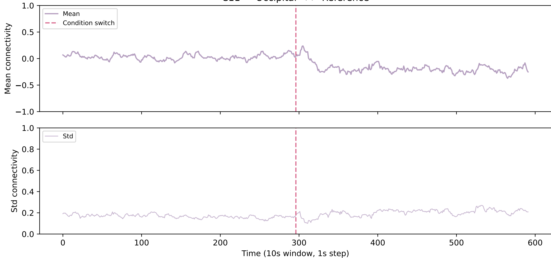
C11 — Occipital <-> Reference
