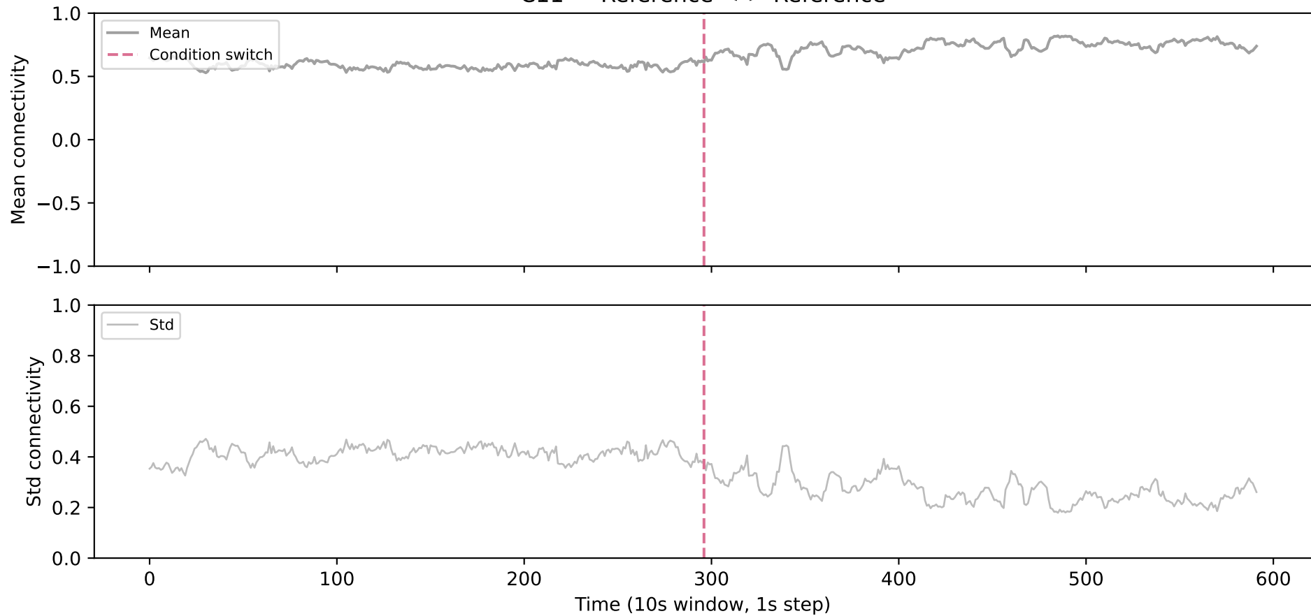
C11 — Reference <-> Reference
