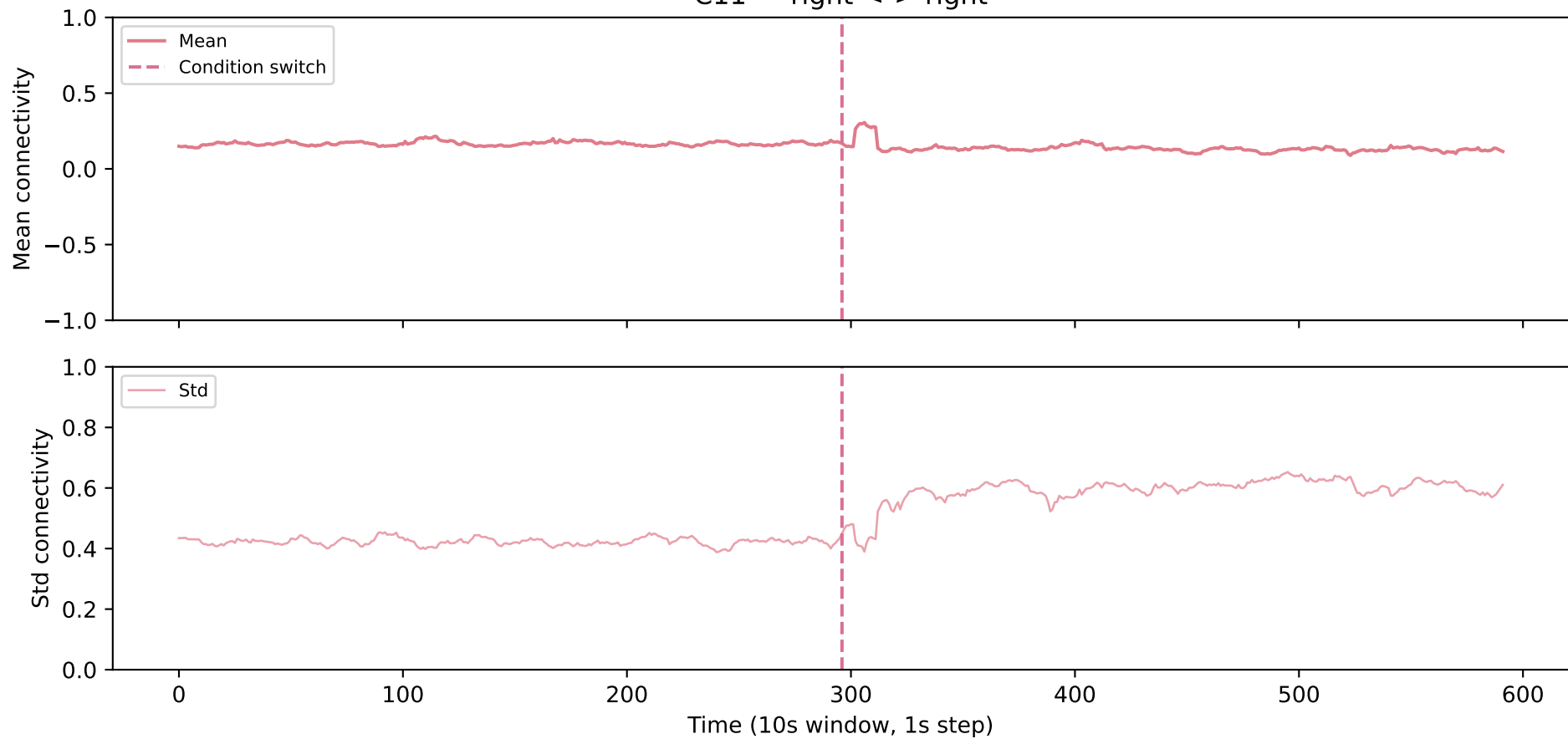
C11 — right <-> right
