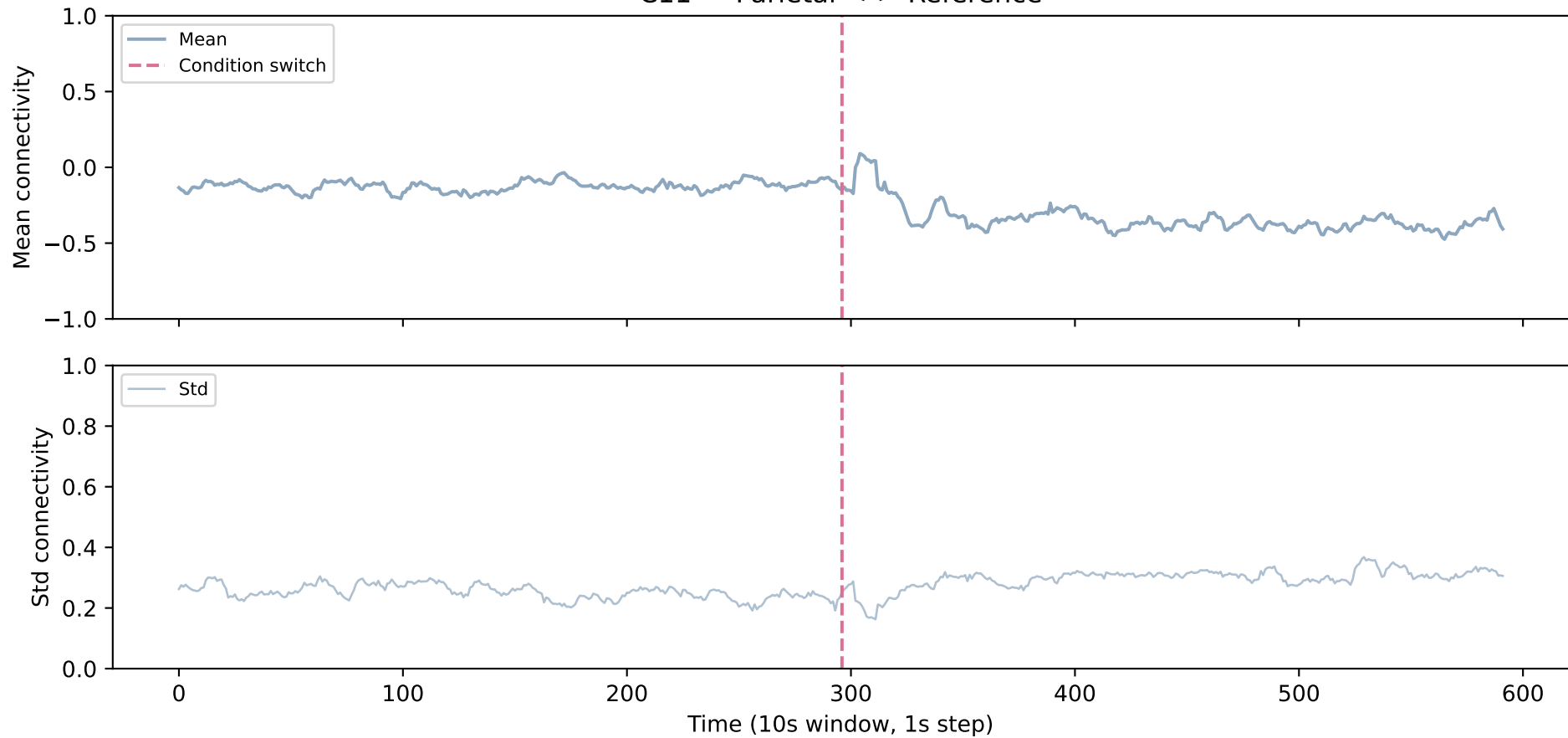
C11 — Parietal <-> Reference
