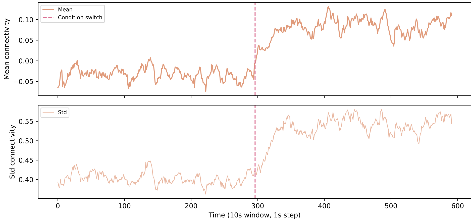
C15 — Frontal <-> Temporal
