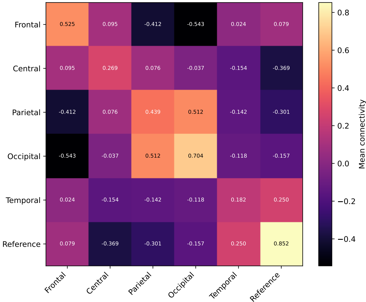
C15 — mean connectivity heatmap
