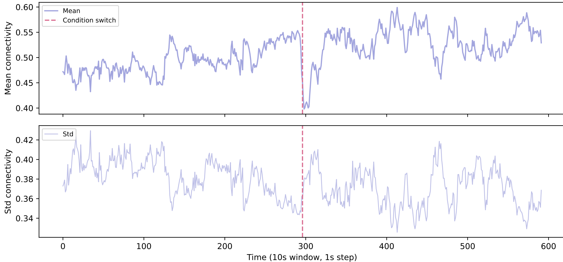
C15 — Parietal <-> Occipital
