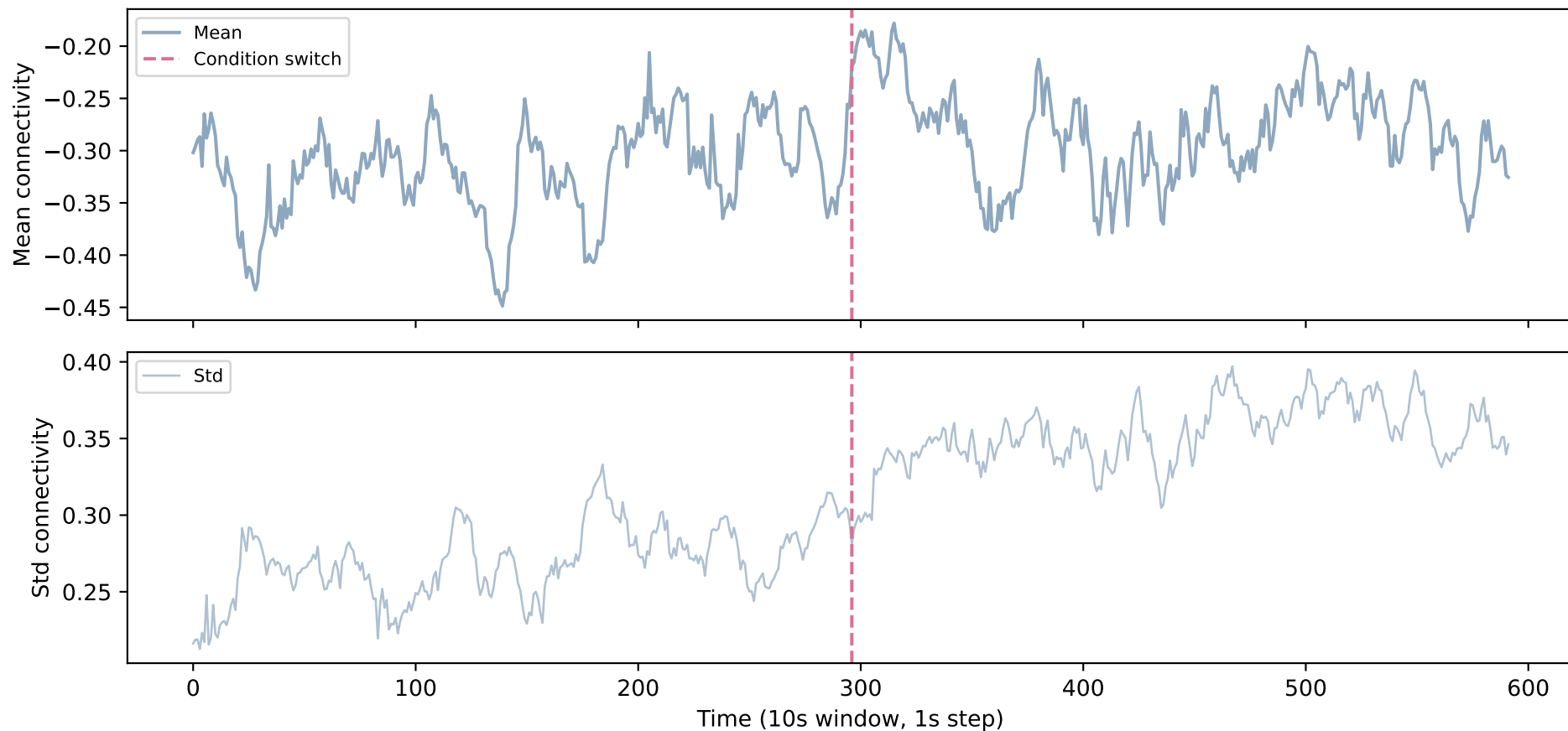
C15 — Parietal <-> Reference
