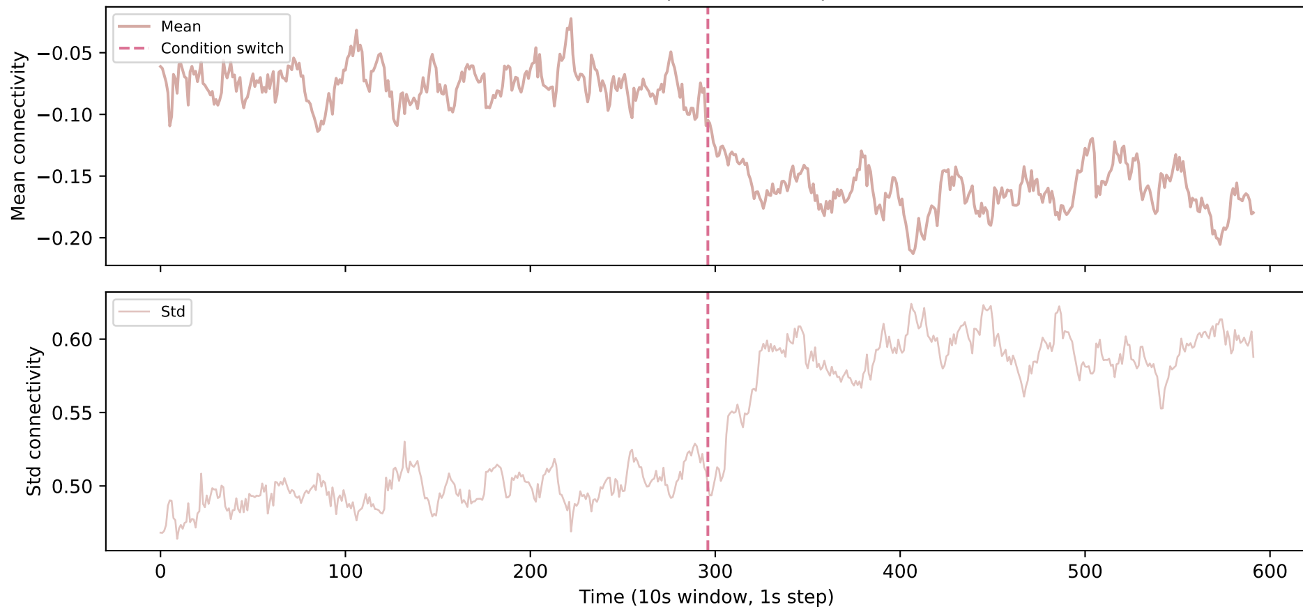
C15 — Occipital <-> Temporal
