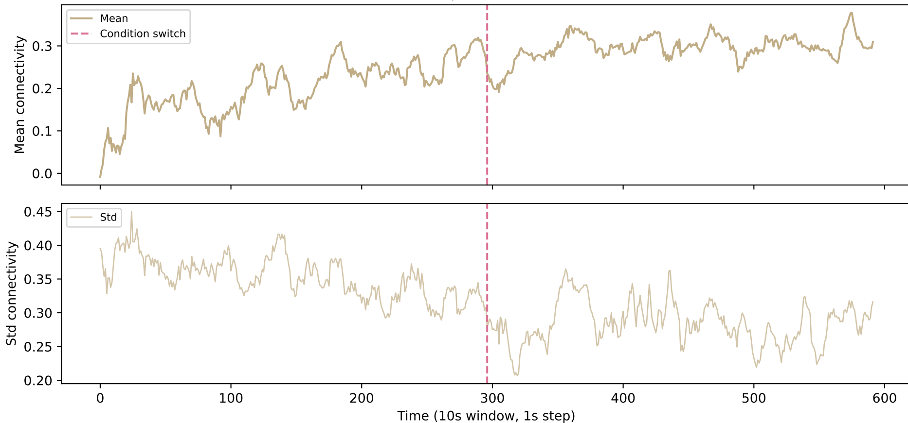
C15 — Temporal \leftrightarrow Reference
