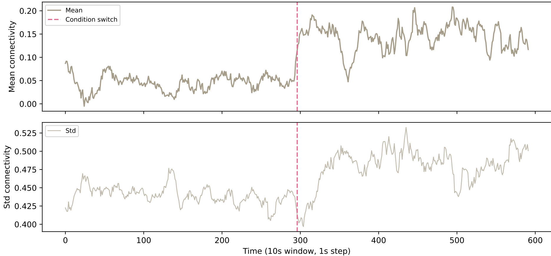
C15 — Frontal <-> Central
