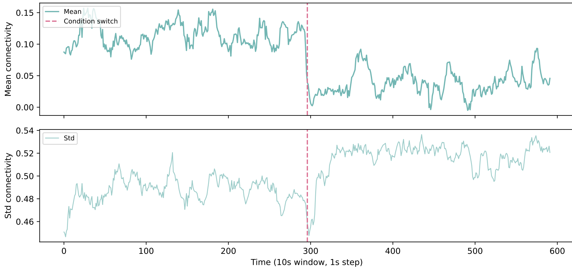
C15 — Central <-> Parietal
