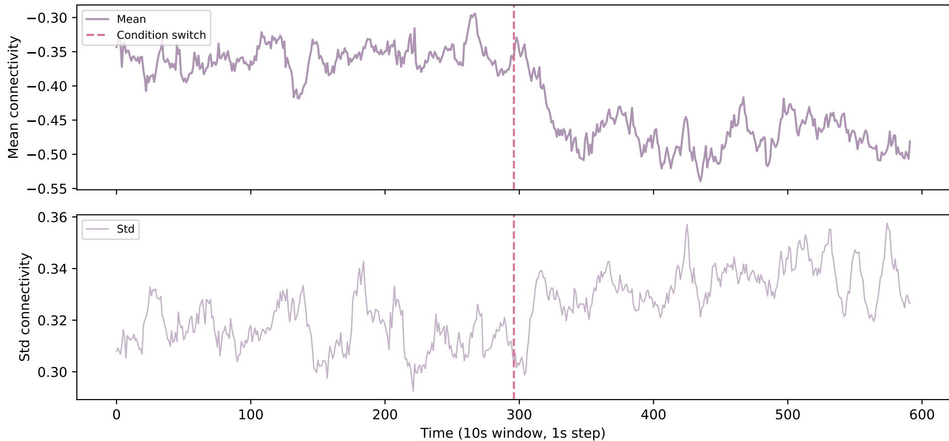
C15 — Frontal <-> Parietal
