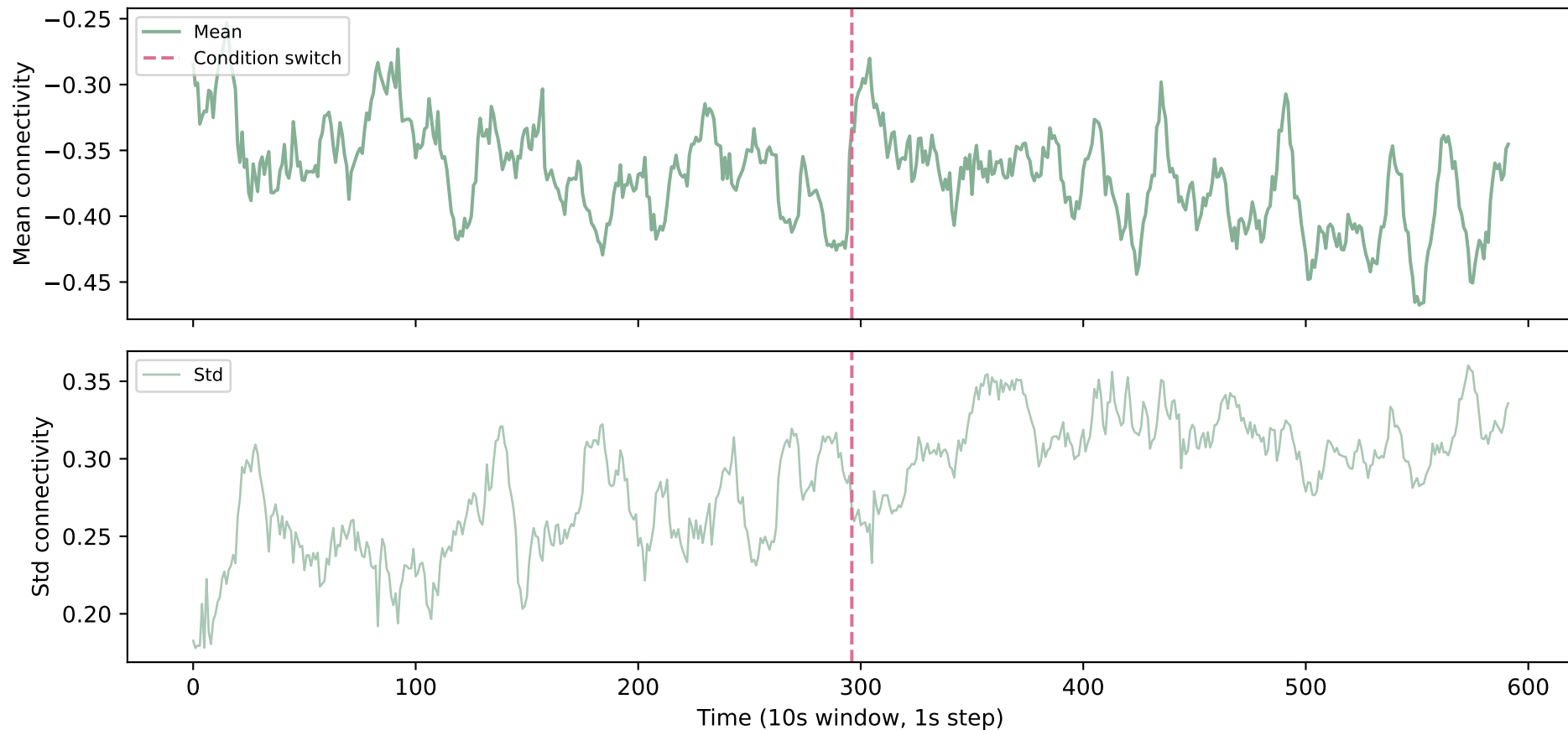
C15 — Central <-> Reference
