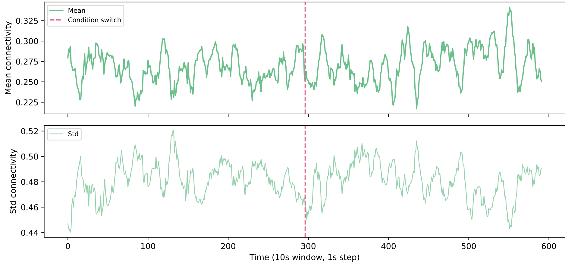
C15 — Central <-> Central
