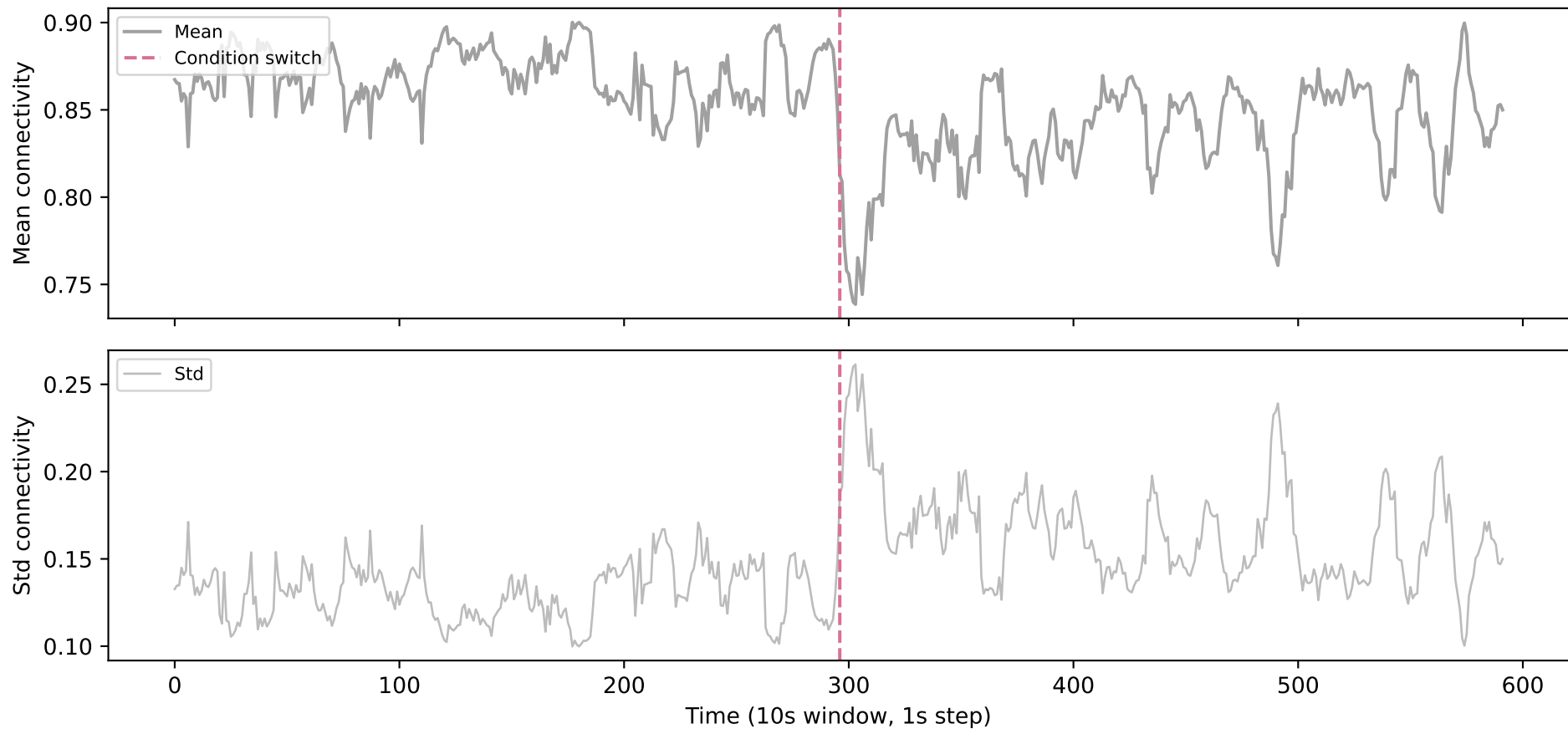
C15 — Reference <-> Reference
