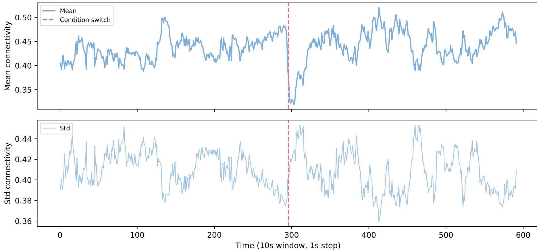
C15 — Parietal <-> Parietal
