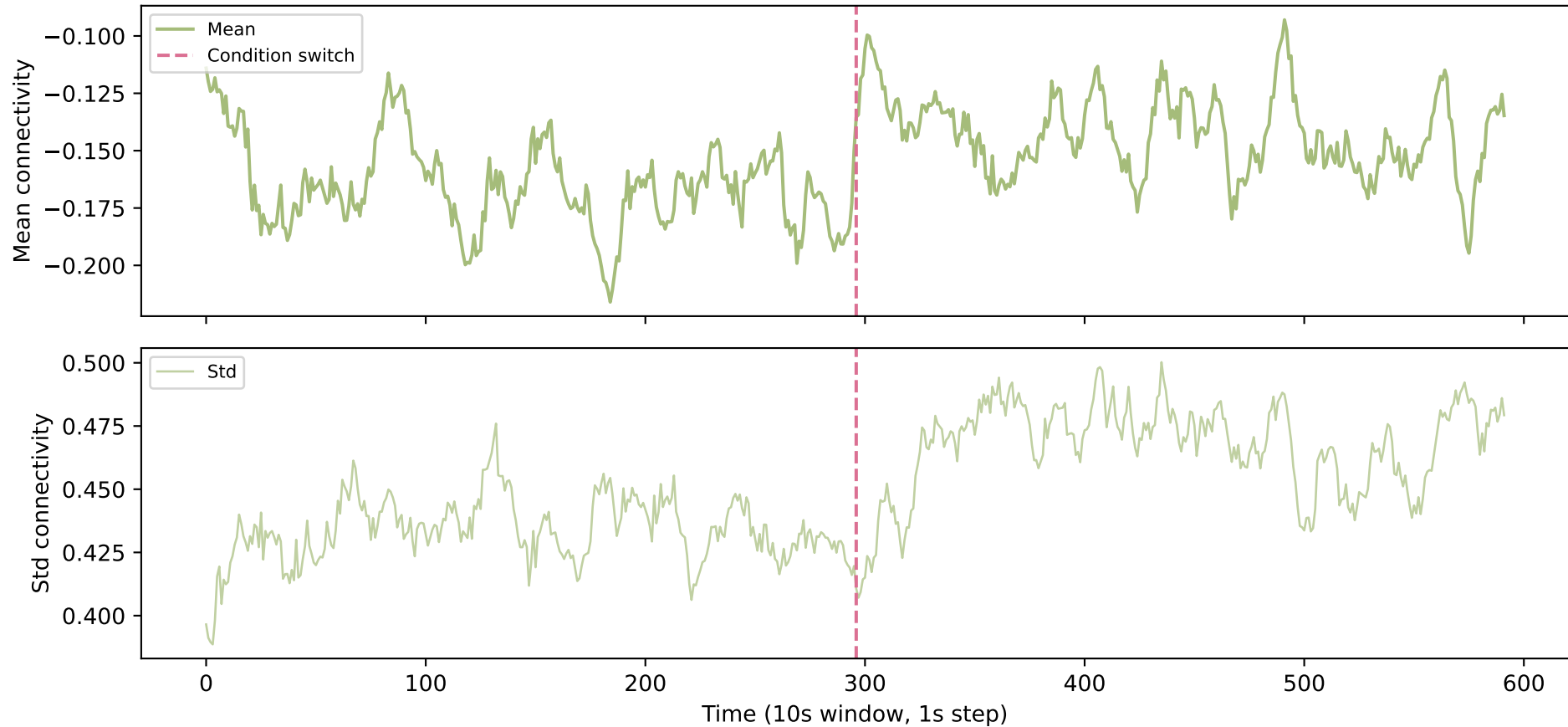
C15 — Central <-> Temporal
