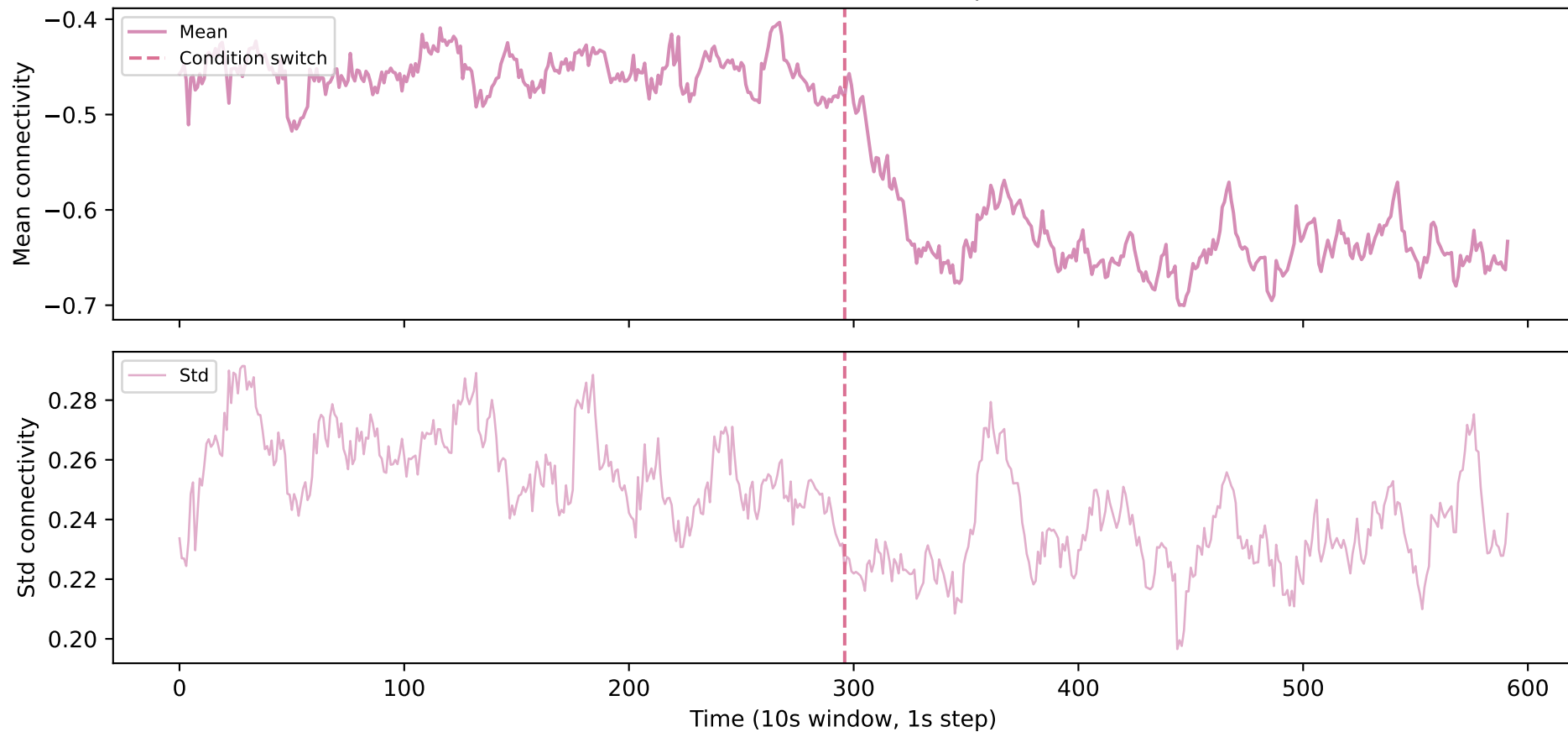
C15 — Frontal <-> Occipital
