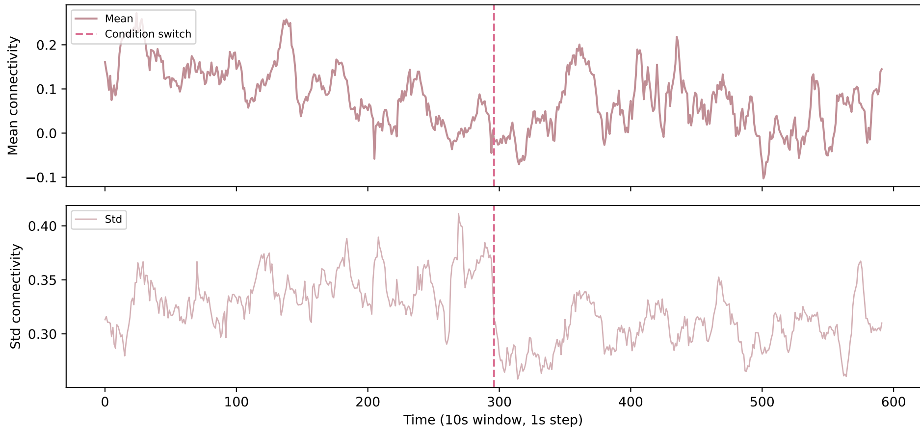
C15 — Frontal <-> Reference
