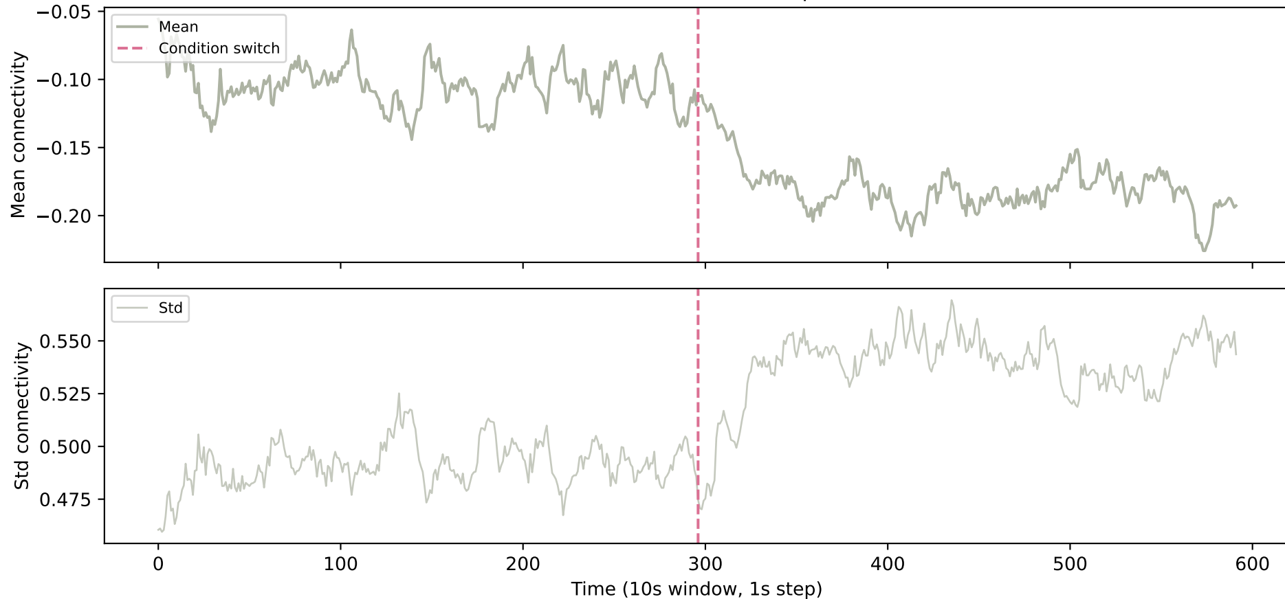
C15 — Parietal <-> Temporal
