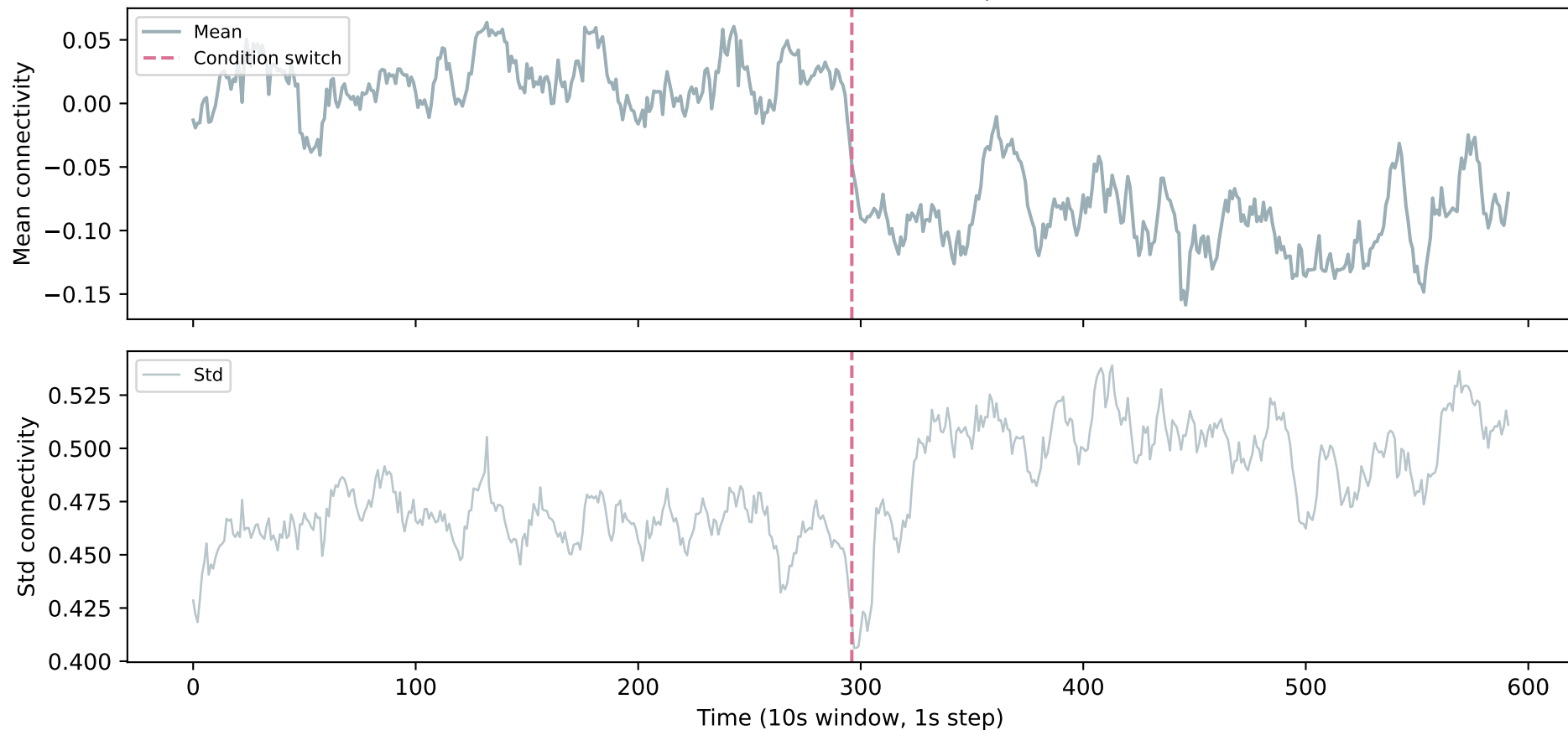
C15 — Central <-> Occipital
