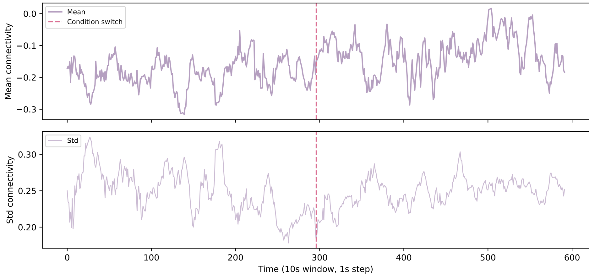
C15 — Occipital <-> Reference
