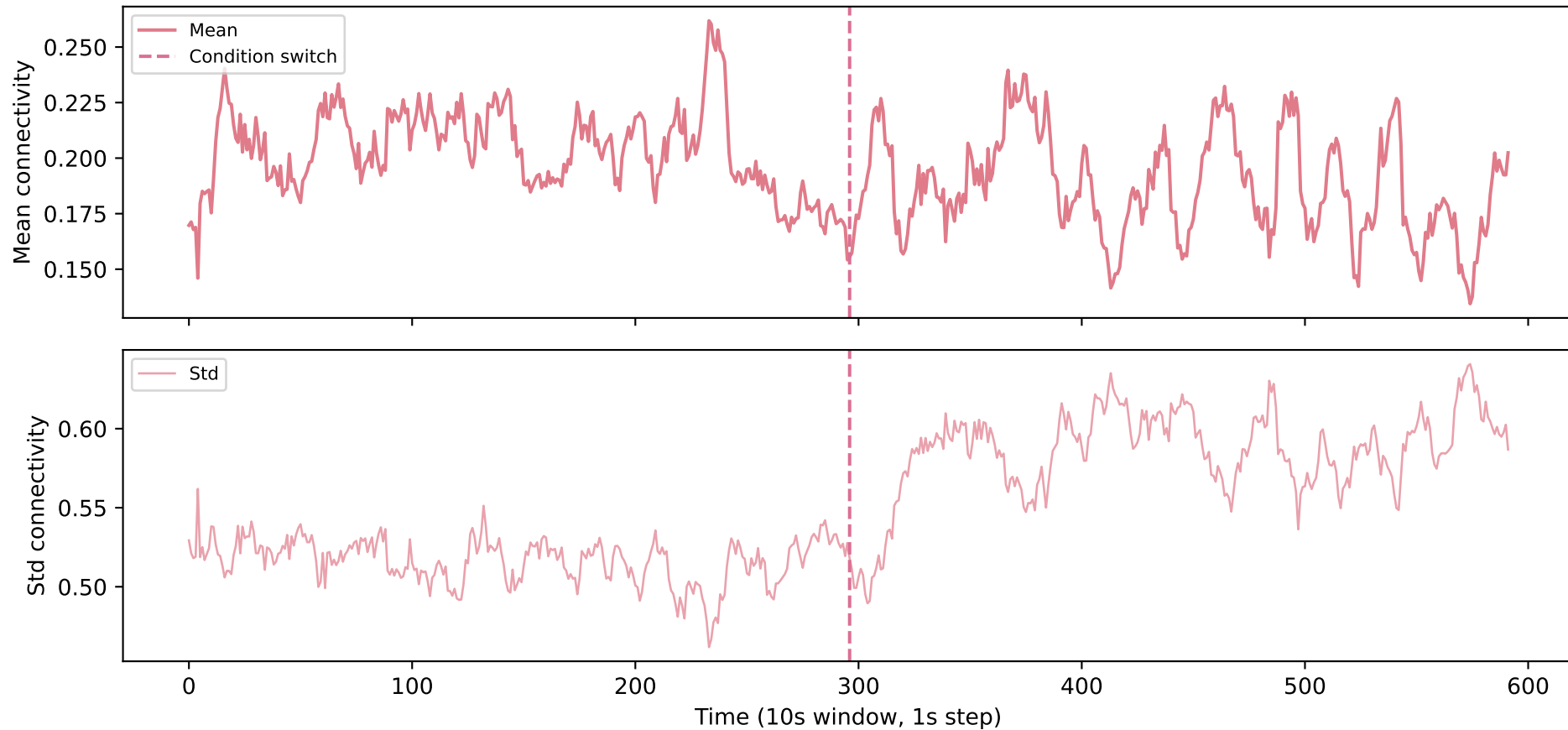
C15 — right <-> right
