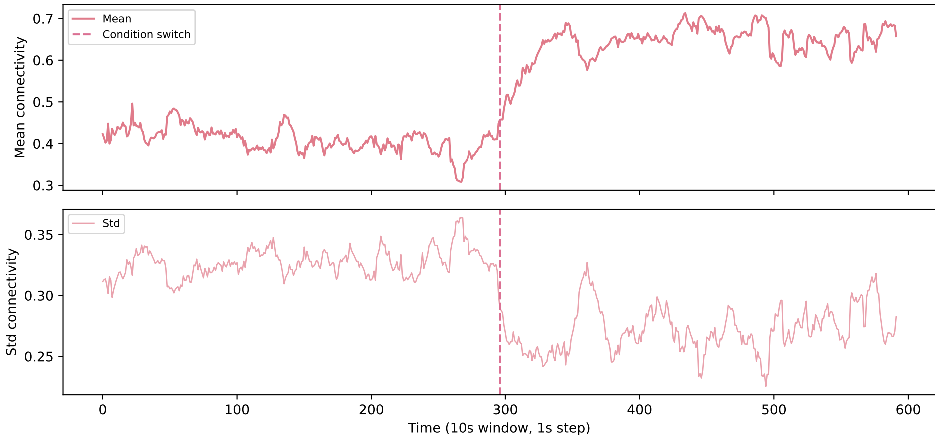
C15 — Frontal <-> Frontal
