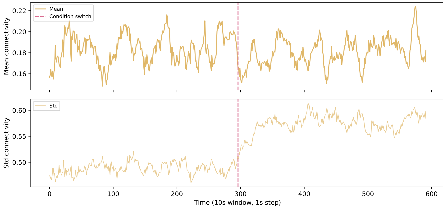
C15 — Temporal <-> Temporal
