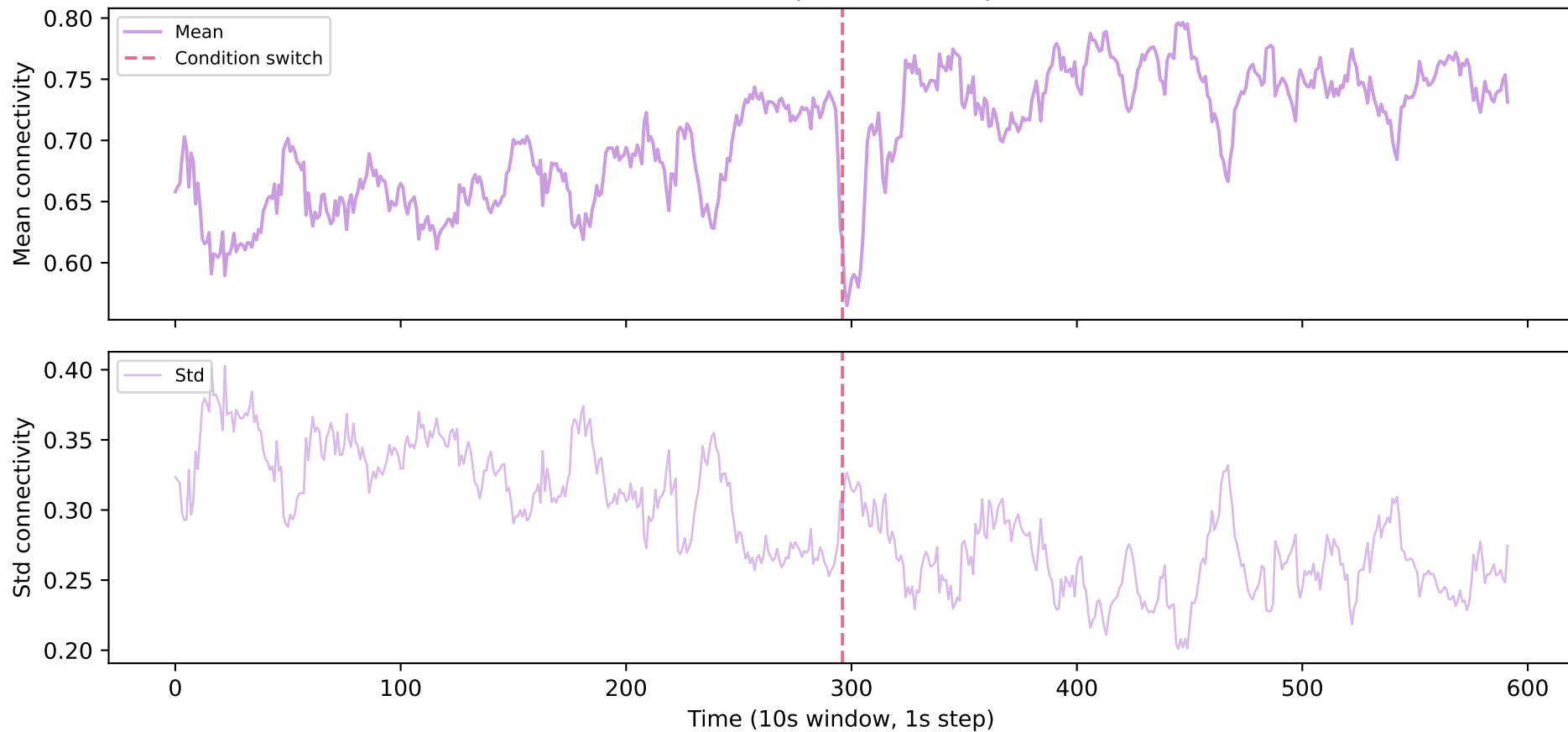
C15 — Occipital <-> Occipital
