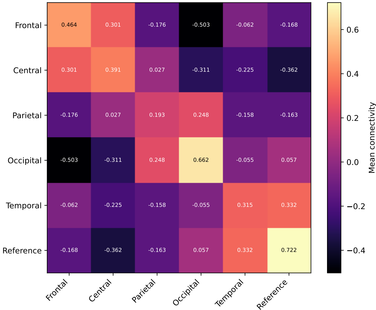
C20 — mean connectivity heatmap
