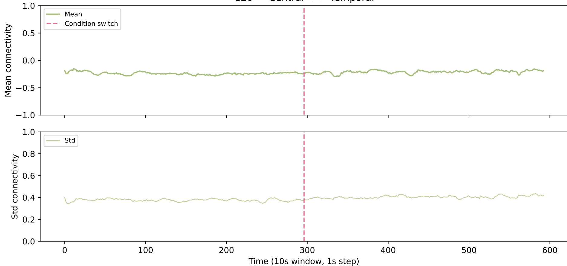
C20 — Central <-> Temporal
