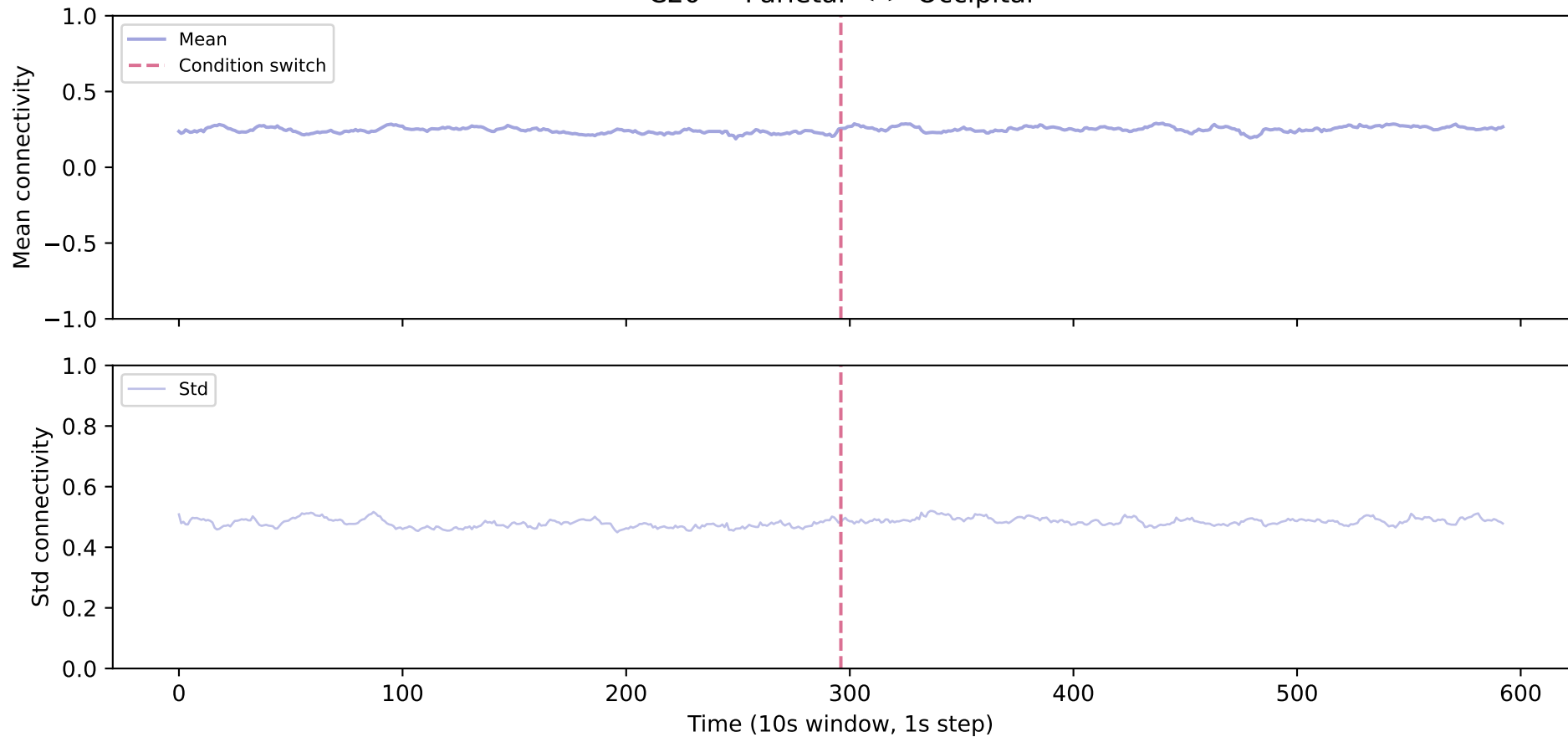
C20 — Parietal <-> Occipital
