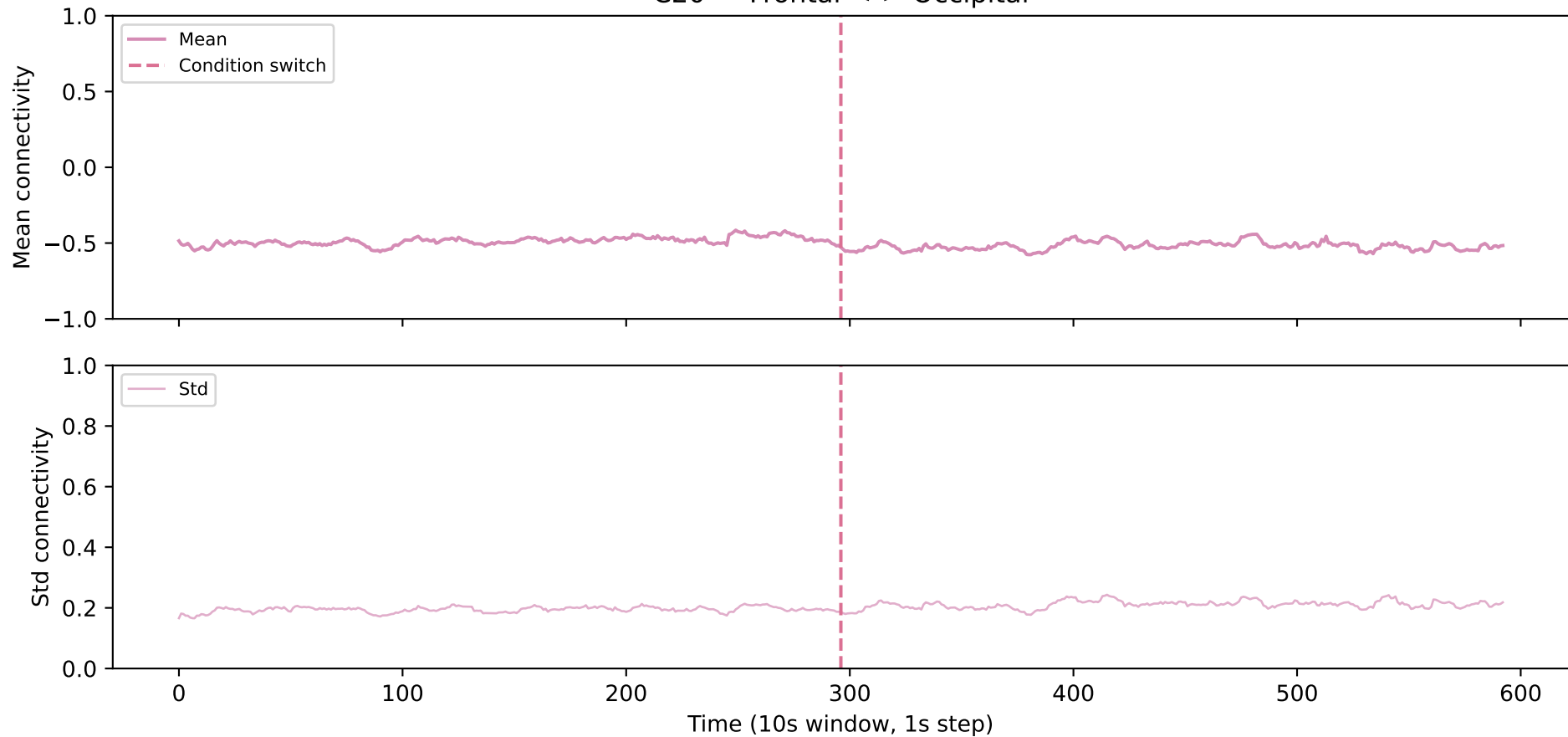
C20 — Frontal <-> Occipital
