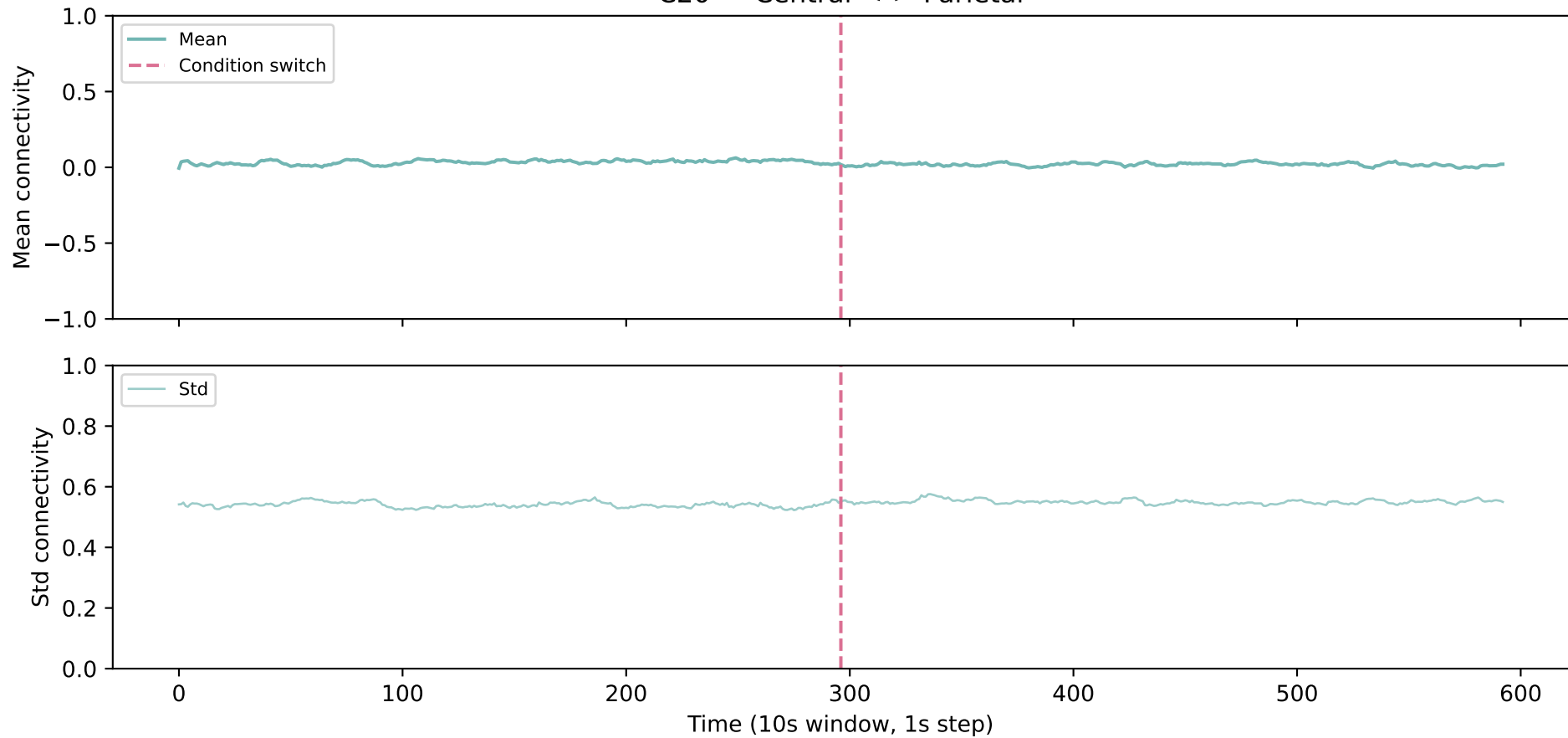
C20 — Central <-> Parietal
