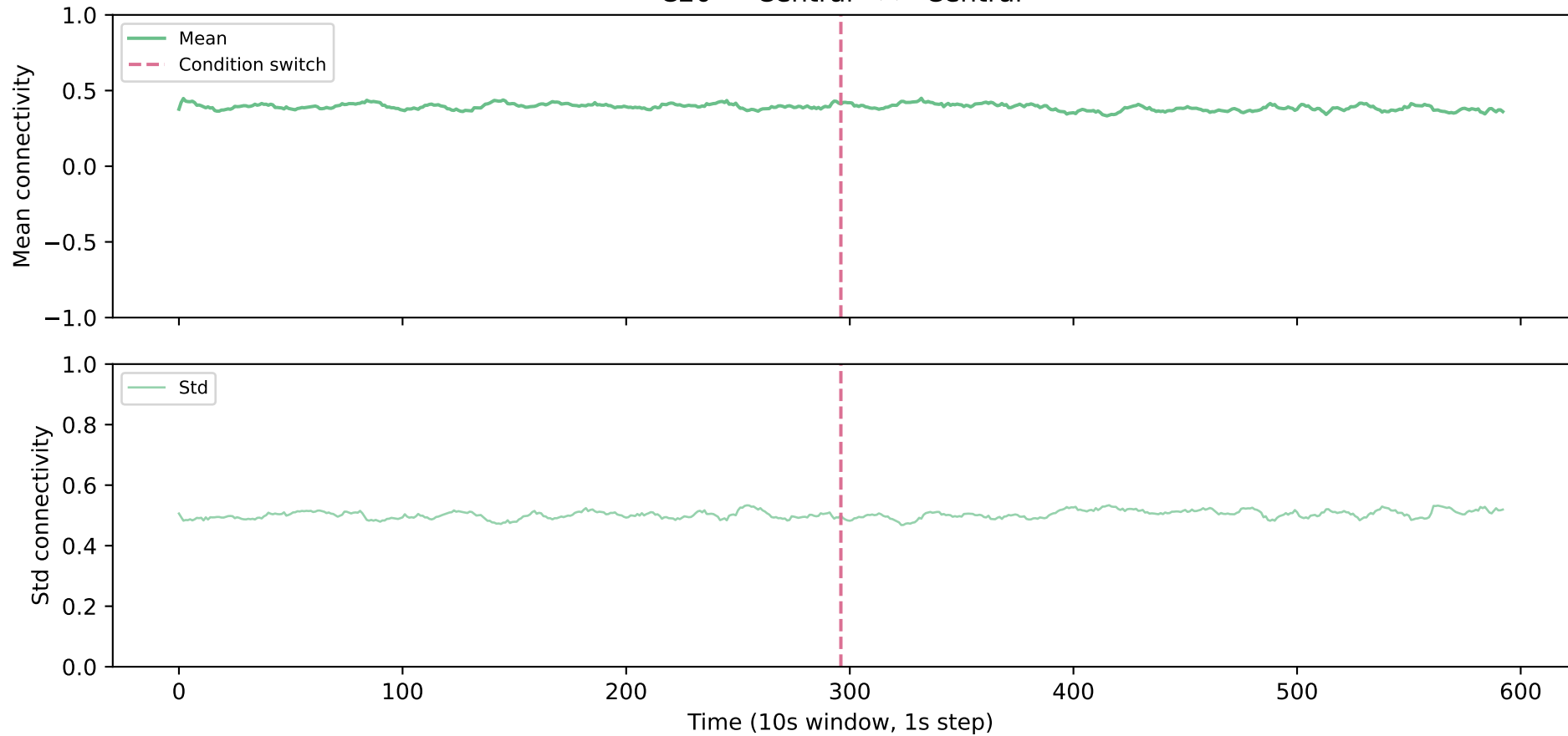
C20 — Central <-> Central
