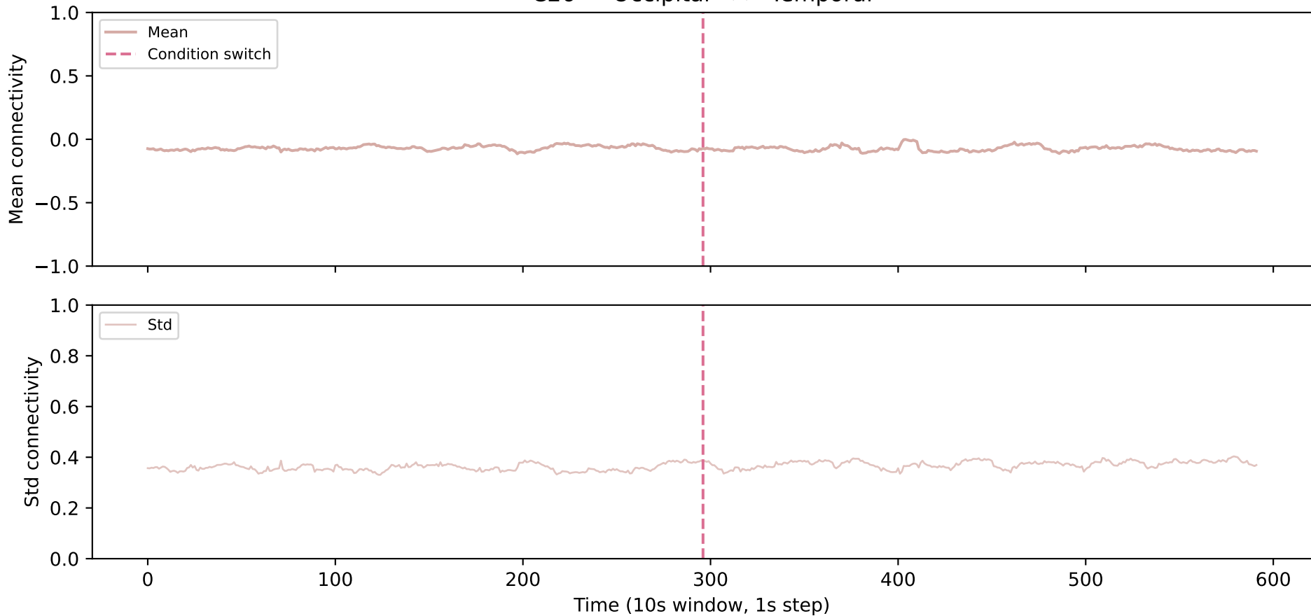
C26 — Occipital <-> Temporal
