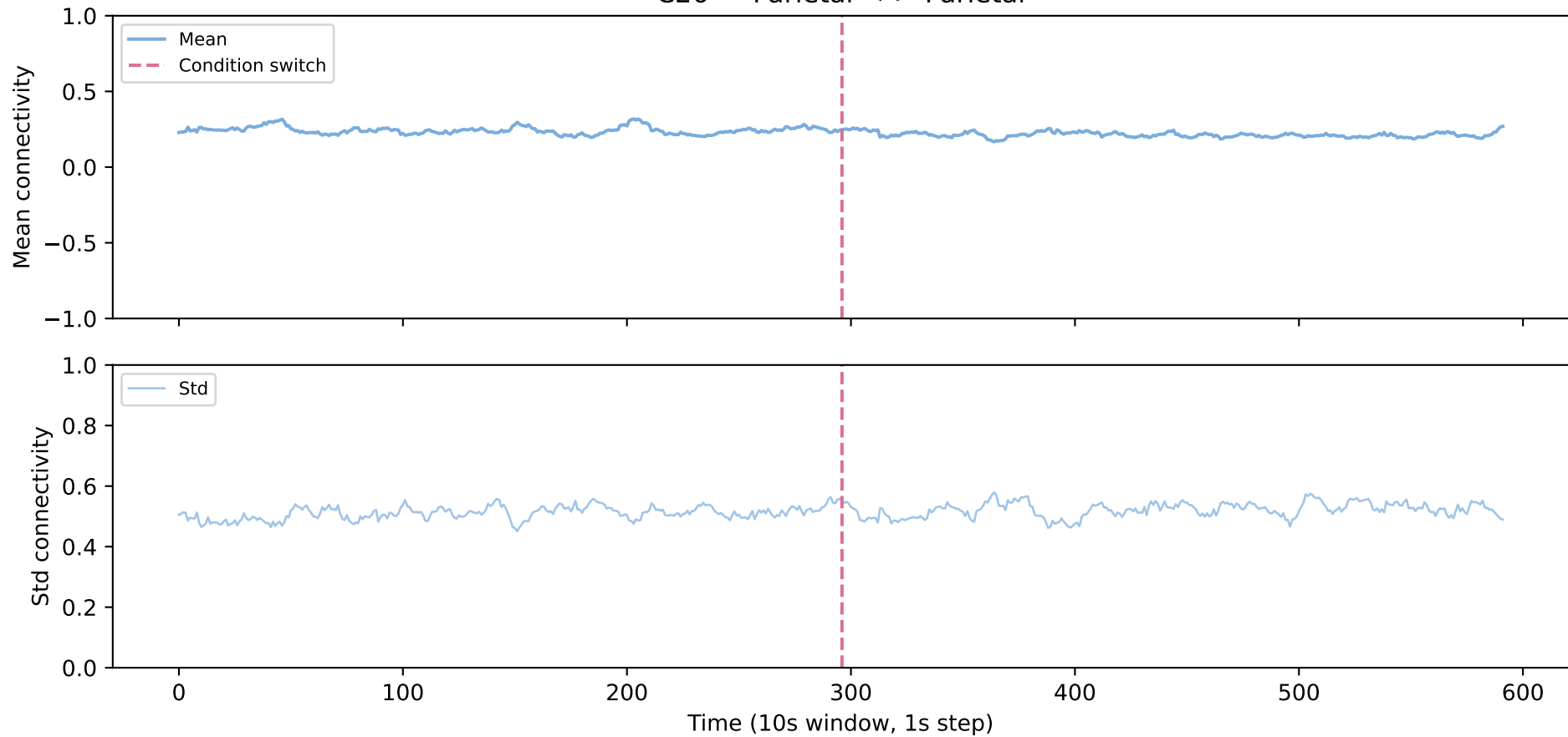
C26 — Parietal <-> Parietal
