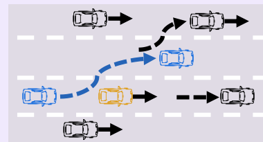
Interaction-aware rollout
