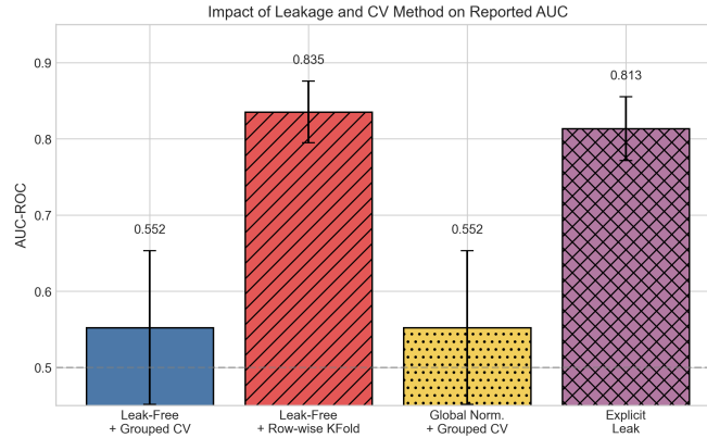
Fig. 1. Main benchmark (30 replicates) under matched five-fold protocols. Row-wise KFold increases AUROC and improves Brier score relative to episode-grouped five-fold validation even though the features are strictly causal.
