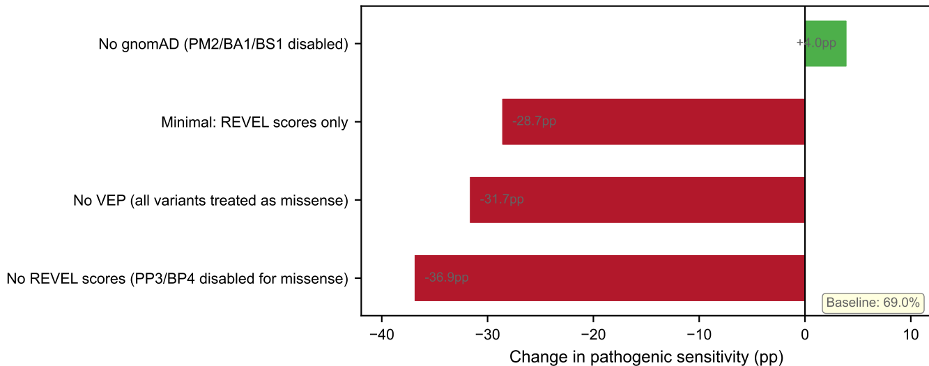
Impact of data source removal on classification sensitivity
