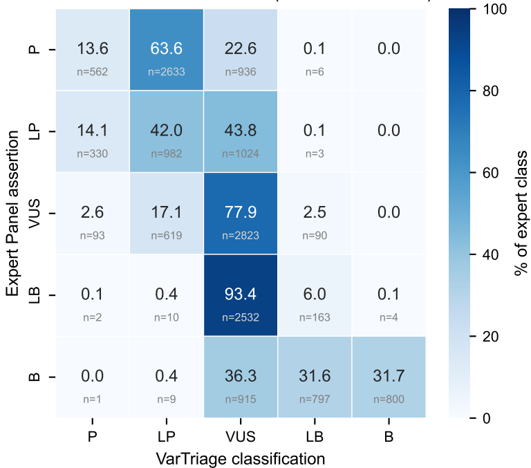
Classification concordance (row-normalized %)
