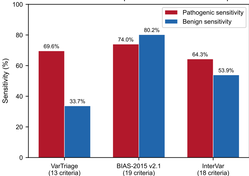
Multi-tool classification performance on ClinGen eRepo
