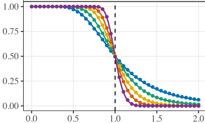
Logistic
