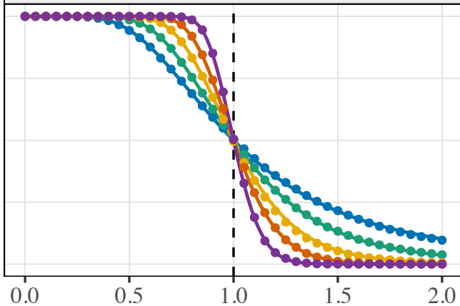
Laplace
