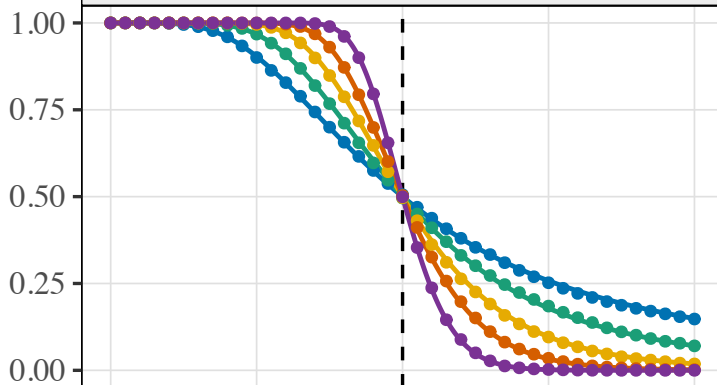
Logistic
