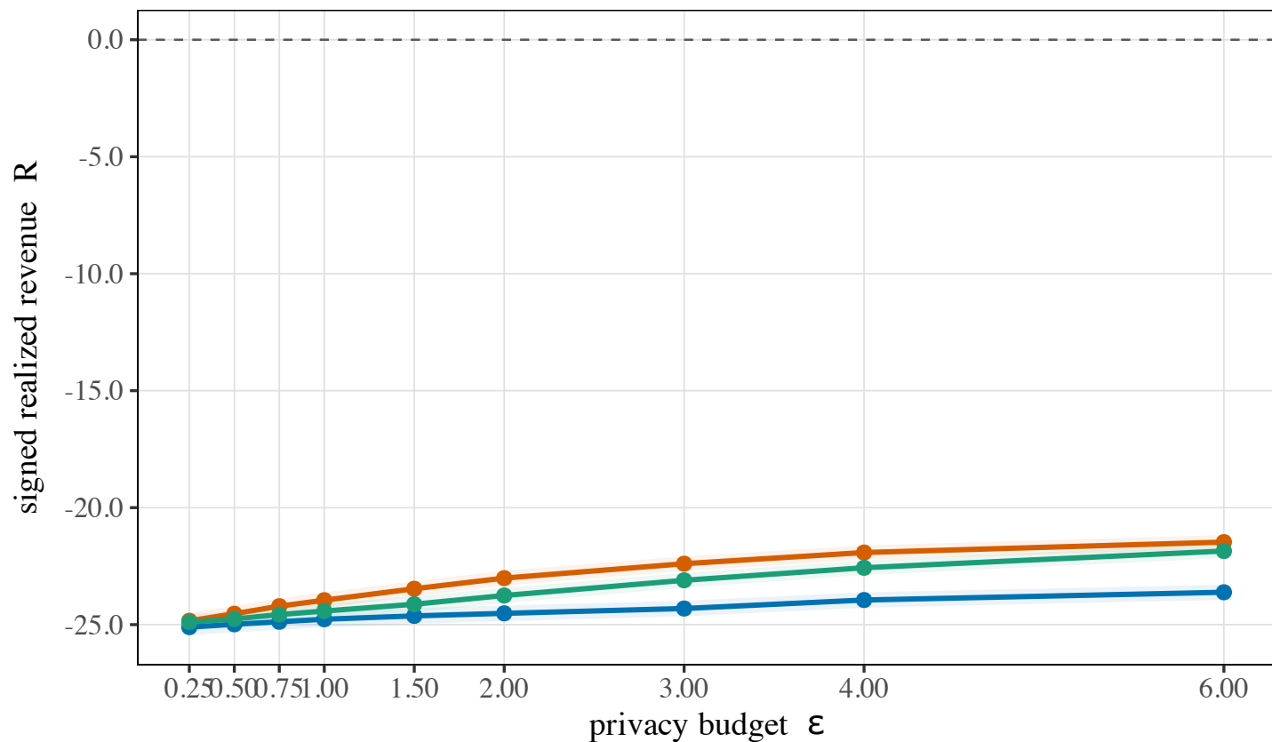
\lambda = 1 ; common (epsilon, delta)-LDP frontier
