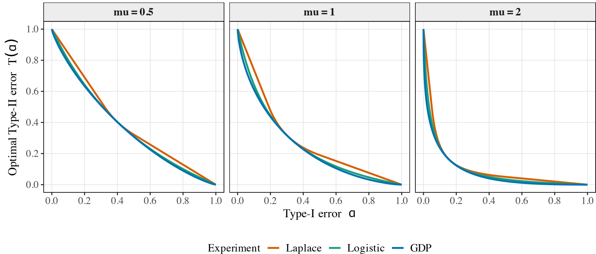
Common tight mu-GDP calibration; the logistic endpoint curve lies weakly below Laplace
