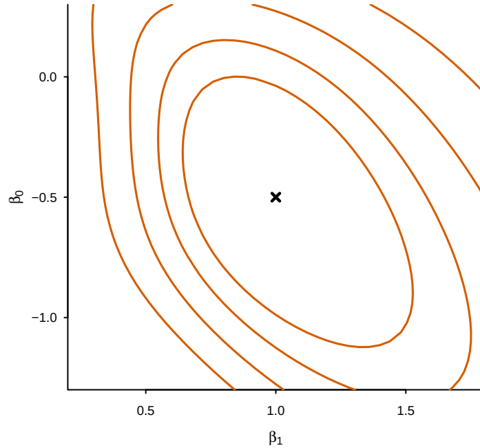
(b) Penalization component
