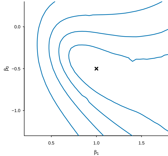
(a) Wald component
