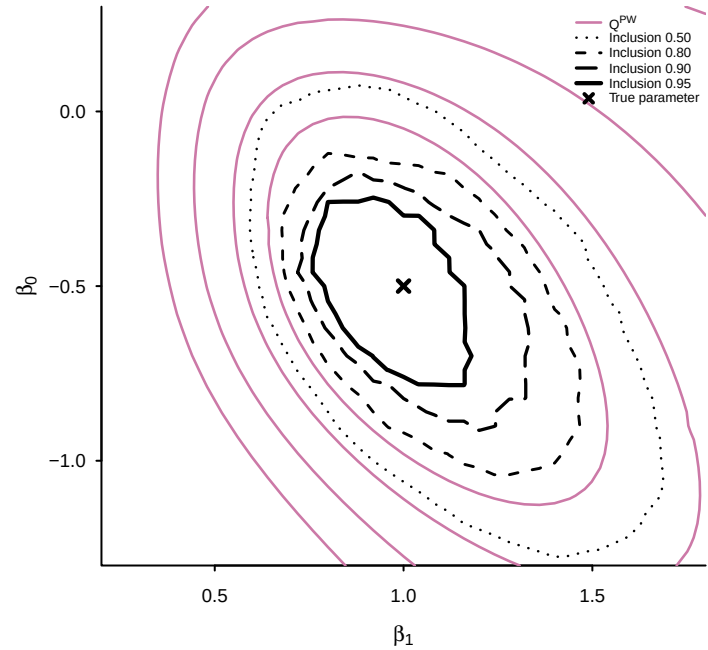
(c) Penalized Wald and Repro set
