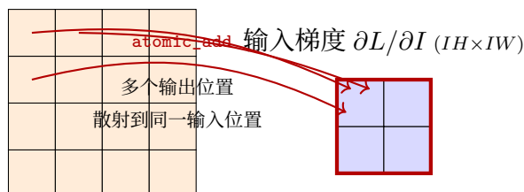
Figure 7 upsample_nearest2d 反向传播的散射示意：多对一映射需原子累加
