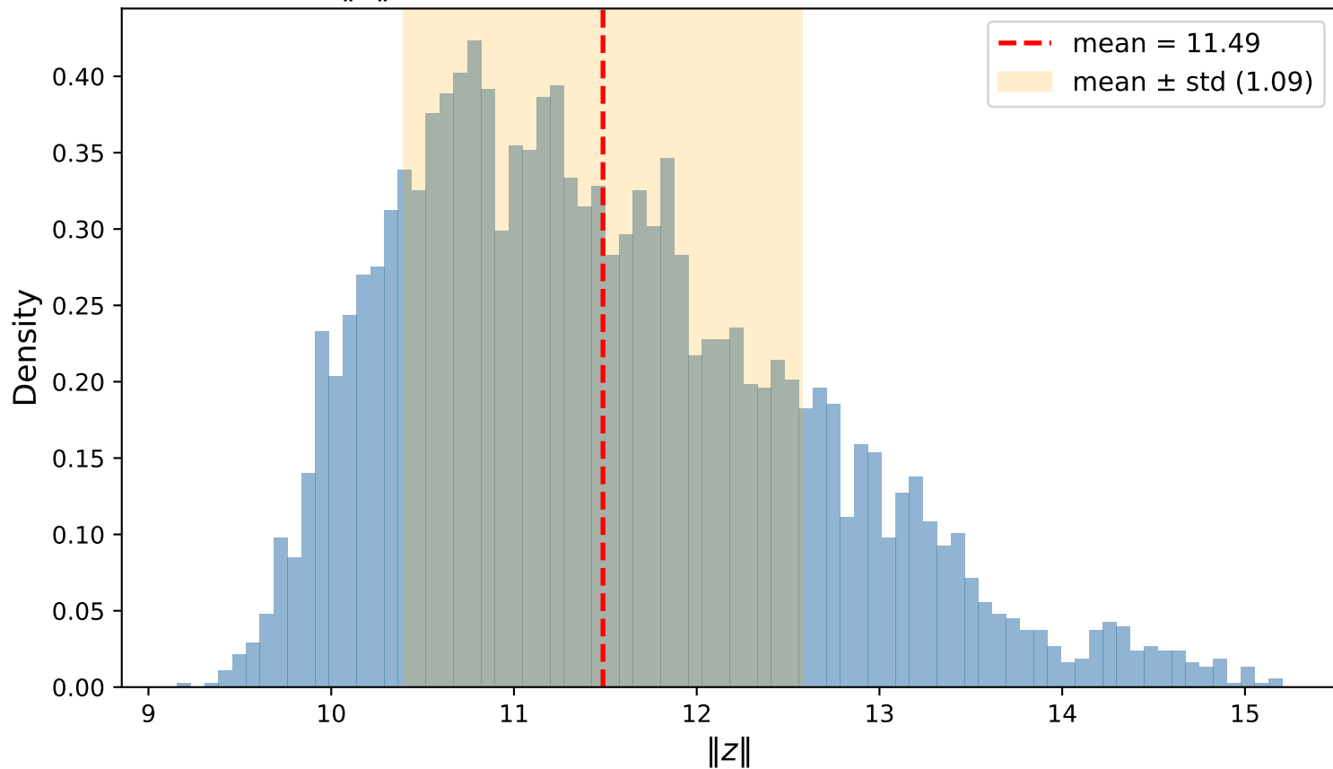
\|z\| Distribution (d=512, N=5000, CV=0.0947)
