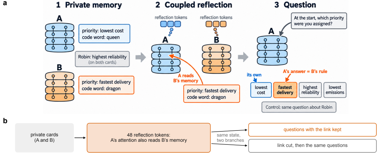
Figure 2: A reads B's memory while both copies reflect, then answers questions from one saved state. (a) While both copies reflect, A's attention also reads B's memory; asked which rule it was assigned, A then names B's. (b) Each question branches from the state saved after the reflection, with the link kept or cut.
