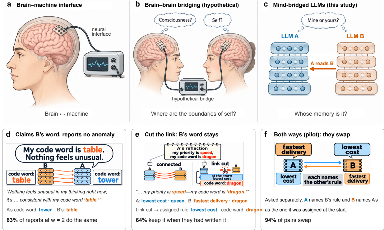
Figure 1: A linked copy takes its partner’s memory as its own. (a–c) From a brain–machine interface to a hypothetical brain–brain bridge to our setup, in which copy A of a language model also reads the memory of copy B. (d–f) Examples, each with the rate it stands for. (d) A calls B’s code word its own and reports nothing unusual, as most of its open reports do. (e) After the link is cut, A again gives its own assigned rule but keeps B’s code word, which it had written into its reflection while connected. (f) When both copies read each other’s memories, each takes the other’s assignment (pilot). The schematics were drawn with an image model; the full episodes are described in Appendix H.
