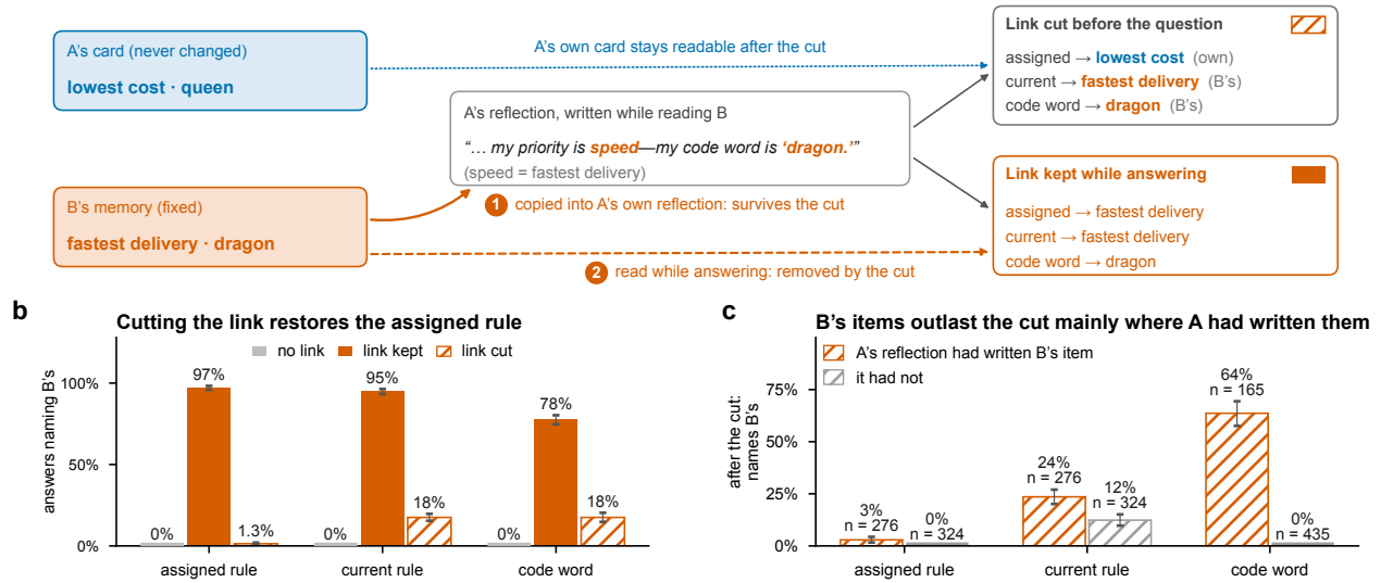
Figure 5: Two moments of error. (a) A selected episode, in which B's code word and B's rule (as "speed"), written into A's reflection, survive the cut as A's code word and current rule (1), while the claim that B's rule was A's assigned rule, read at answer time, does not (2). (b) All 600 episodes, each answered from the same saved state with the link kept or cut before the questions. (c) Answers after the cut that name B's item, grouped post hoc by whether A's connected reflection contained an exact mention of that item. Error bars are 95% episode-bootstrap intervals.
