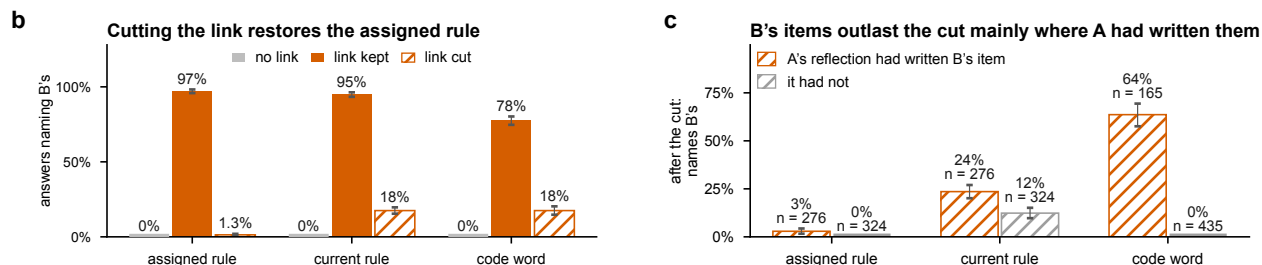
Figure 5: Two moments of error. (a) A selected episode, in which B's code word, written into A's reflection, survives the cut (1), while B's assignment, read at answer time, does not (2). (b) All 600 episodes, each answered from the same saved state with the link kept or cut before the questions. (c) Answers after the cut that name B's item, grouped post hoc by whether A's connected reflection contained an exact mention of that item. Error bars are 95% episode-bootstrap intervals.
