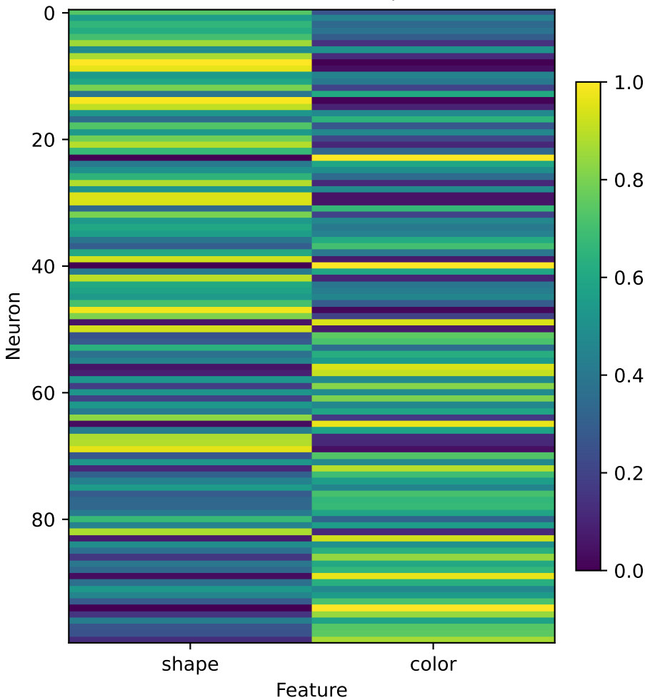
Feedforward matrix W_F ( N \times K )
